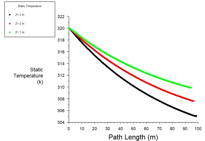
Fig. 14 the outlet water temperature for various soil depths.
