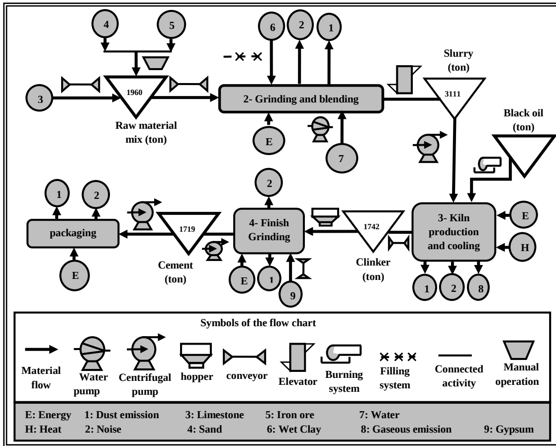
Figure (2) Flow Chart of AL-Kufa Wet Cement Manufacturing
