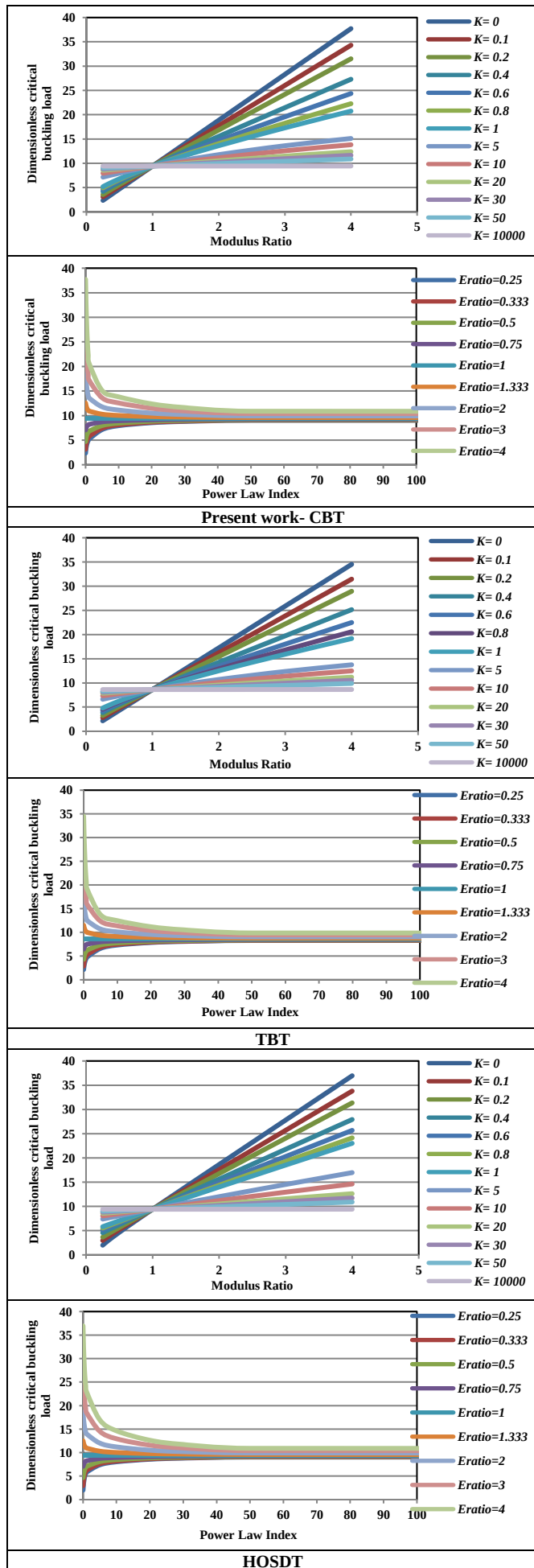
Fig. 5 The effect of modulus ratio and power index dimensionless critical buckling load of FG beam with ( L/H = 5 ) and all theories.
