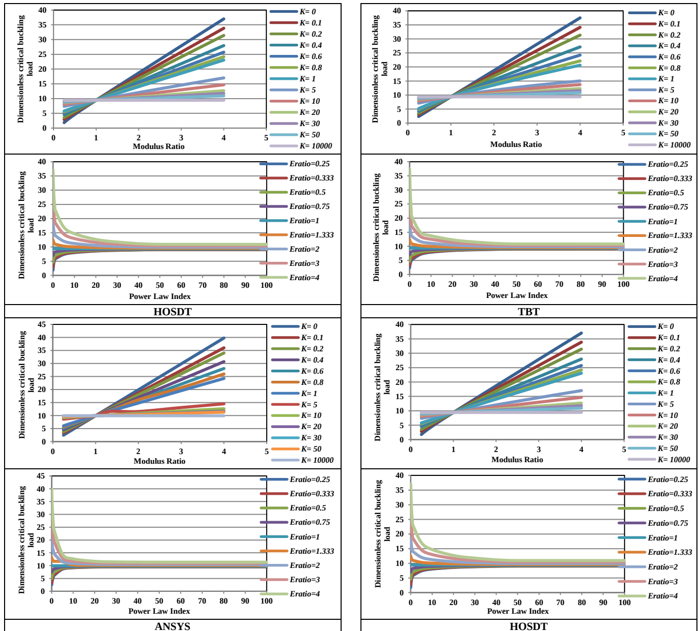
Fig. 6 The effect of modulus ratio and power index on dimensionless critical buckling load of FG beam with aspect ratio 10 and all theories.
