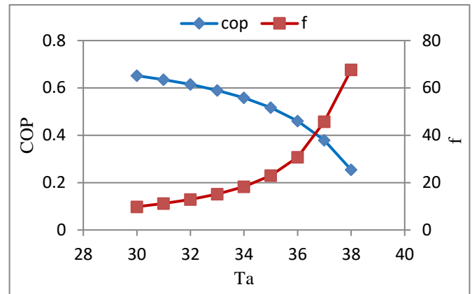
Fig. 12 COP of the absorption cooling system and the circulation ratio with absorber temperature at ( T_g = 70 , T_c = 30 and T_e = 0 ).
