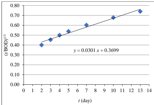
Fig. 13 (t/BOD)^{1/3} versus t for sample No.5
