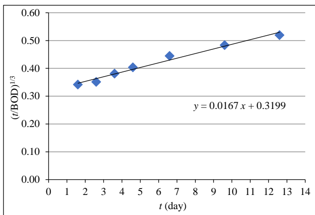
Fig. 7 (t/BOD)^{1/3} versus t for sample No.2
