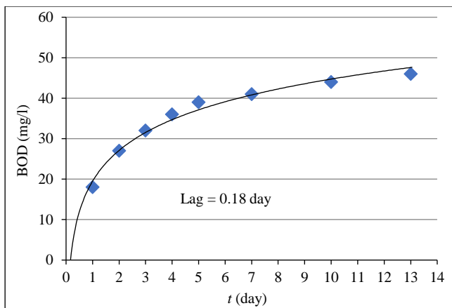
Fig. 14 BOD versus t for sample No.6
