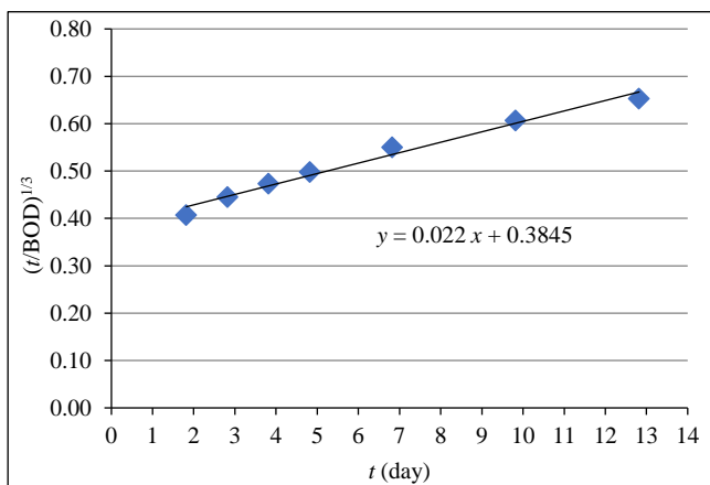
Fig. 15 (t/BOD)^{1/3} versus t for sample No.6
