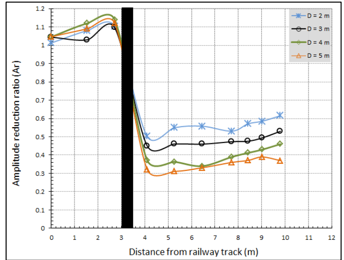
Fig. 10 Efficacy of active isolation using open-trenches with various depths (trench dimensions = 0.4 m \times 10 m, train speed = 120 km/hr).
