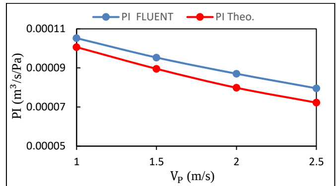
Fig. 34 Variation of productivity index with perforation velocity.
