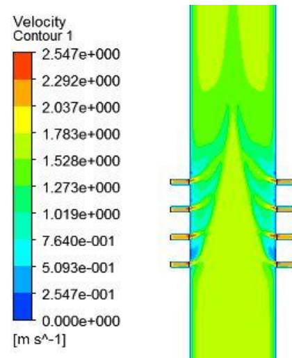
Fig. 10 Velocity contour for 8 perforations with 180° phase angle.
