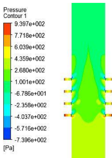
Fig. 13 Pressure contour for 8 perforations with 180° phase angle.
