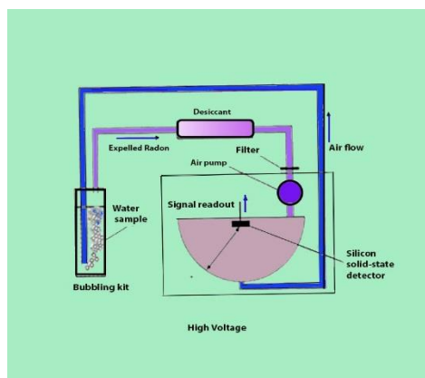
Figure (2) on the right is a picture of the RAD7 device used to measure radon in water models, and on the left is the RADH2O diagram.
