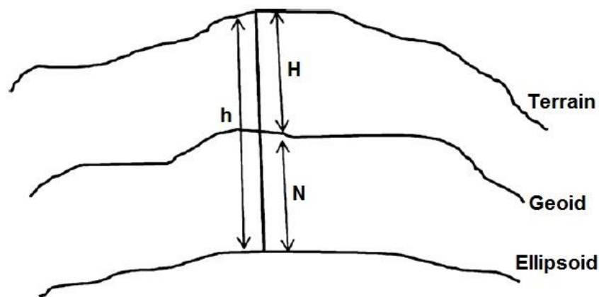
Fig.3: Relation between ellipsoid, geoid and topographic surfaces
