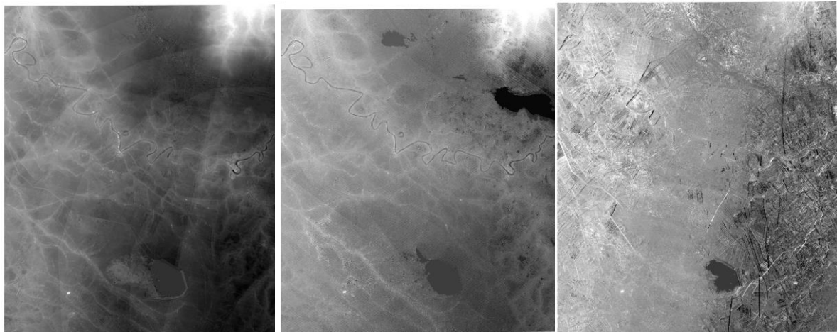
SRTM
