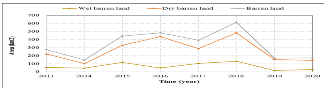
Figure 9: Variability of barren land class
