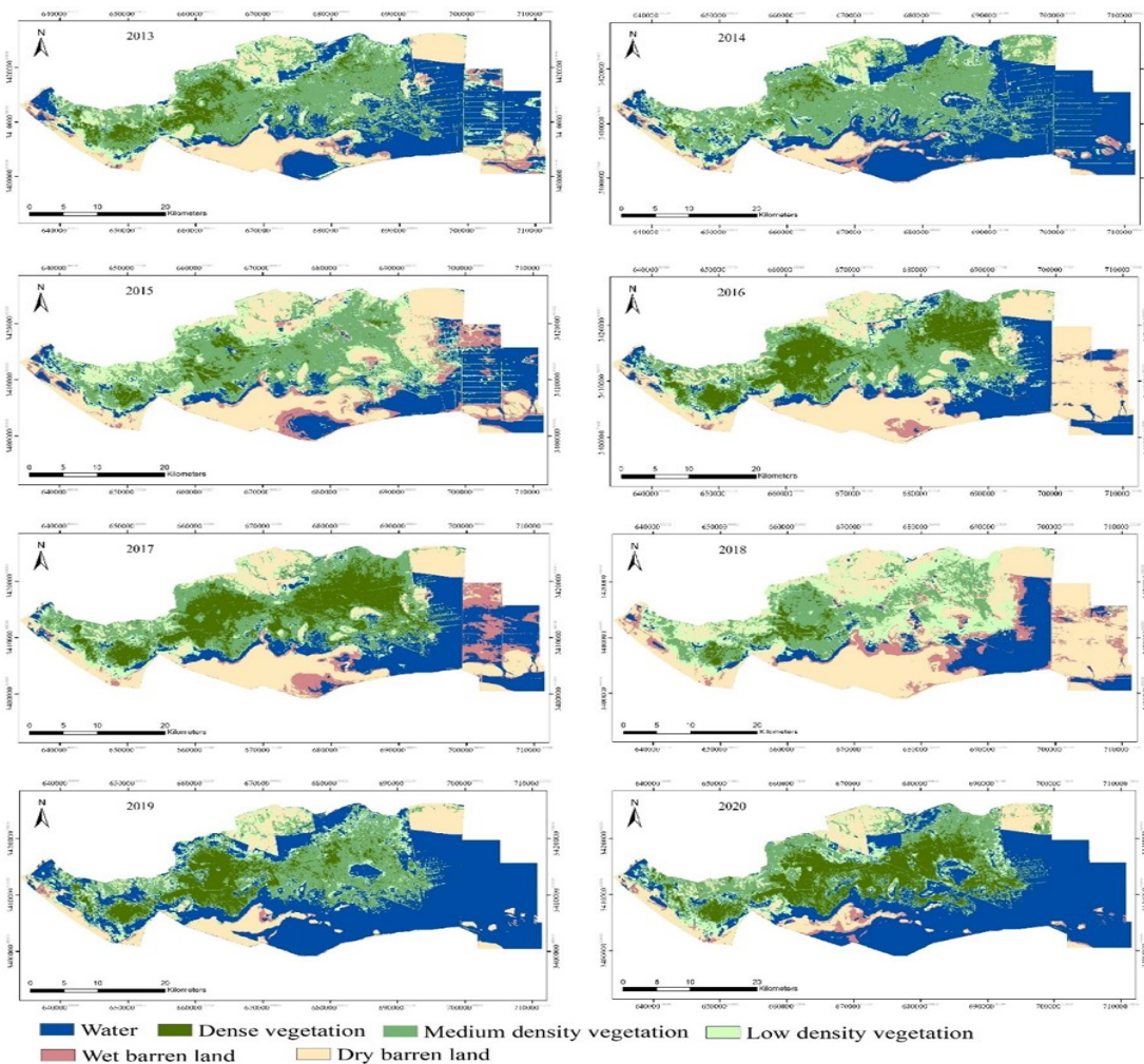
Figure 6: Land cover Categories of Western part of the Al-Hammar Marsh obtained from satellite Images-Based Indices Model
