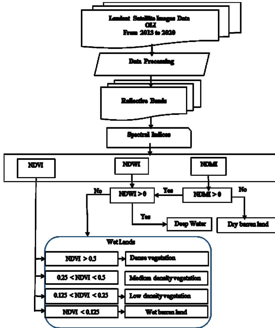
Figure 3: Schematic diagram of the marshland cover classification
