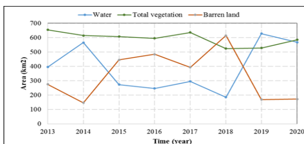
Figure 7: Variability of the land cover classes
