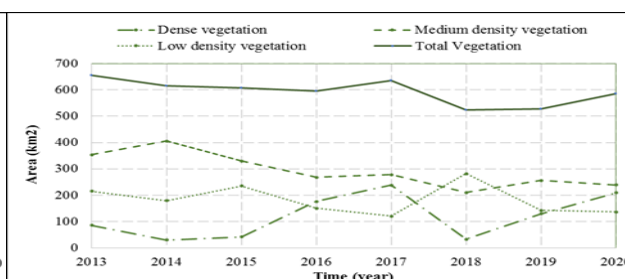
Figure 8: Variability of vegetation cover
