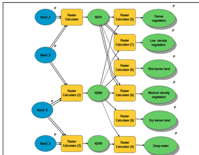
Figure 4: Model builder to classify the land cover of western part of the Al-Hammar Marsh
