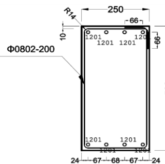
Figure 6: Longitudinal beam
