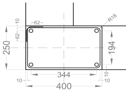
Figure 5: Column cross section
