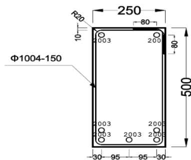
Figure 7: Transverse beam
