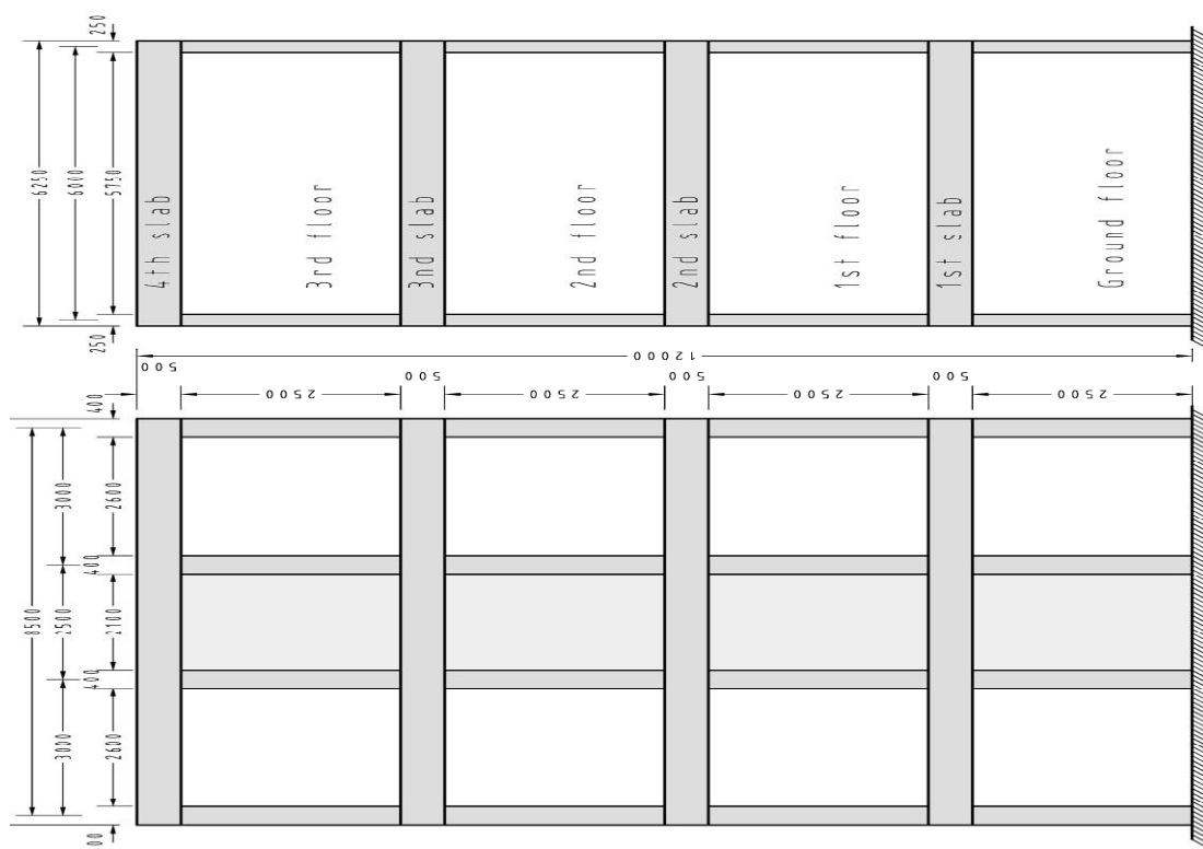
Figure 2: SERFIN specimen Side view with infill wall test model.
