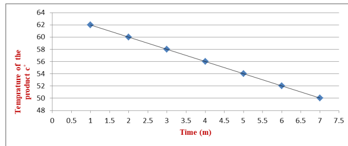
Figure 7: Relation between temperature reductions of product (litter of milk) with time at primary pressure 1.8 bar.
