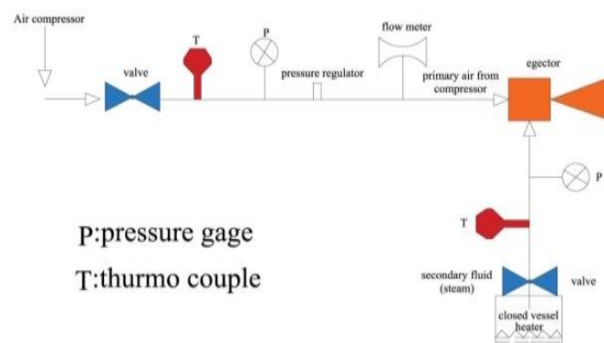
Figure 5: Schematic diagram of system
