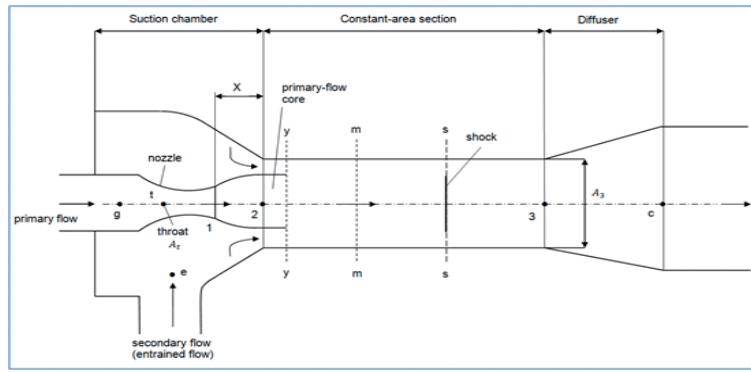
Figure 3: Parts of the ejector according to the above equations [9].
