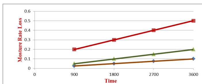
Figure 6: The relation between moisture rate loss and time due to evaporation at different primary pressure (1.8, 1, and 0.5) bar.
