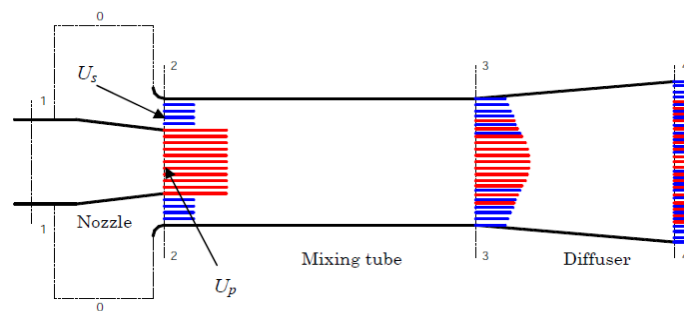
Figure 1: Schematic diagram of an ejector
