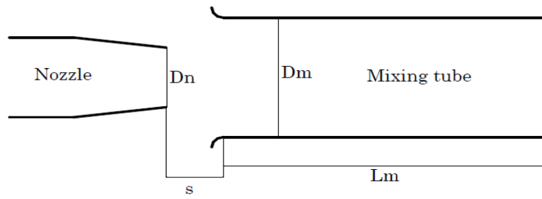
Figure 2: Ejector geometry parameters
