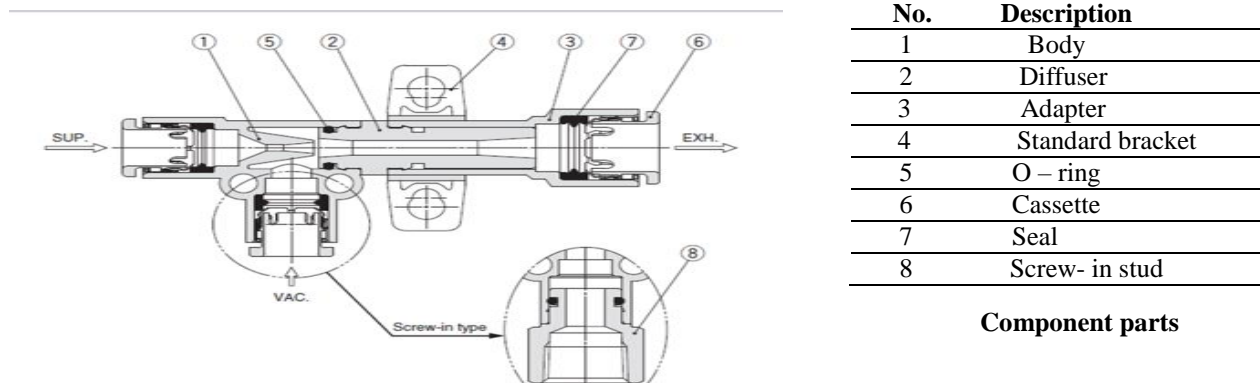
Figure 4: Parts of the ejector
