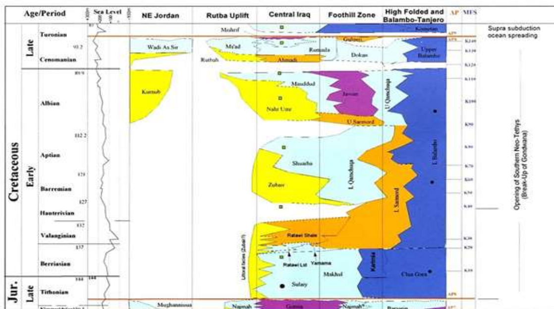
(Fig.2) Regional stratigraphic correlation of Lower Cretaceous units in Megasequence AP8 (Jassim and Goff, 2006)
