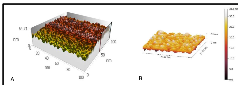
Figure 1: 3D AFM topographical micrograph for nanoparticles of prepared colloidal suspension at 100nm and 50nm respectively.
