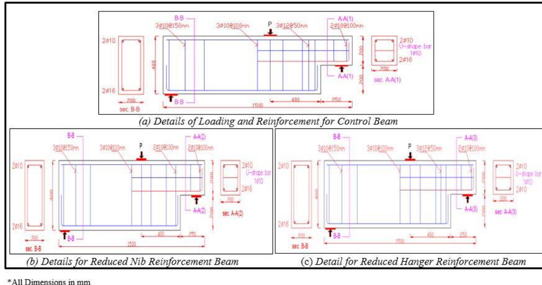
Figure (1) Details of Reinforcement Beams
