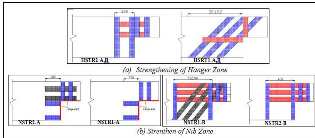
Figure (2) Strengthening Configurations of Dapped end Beams
