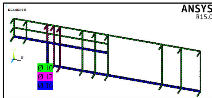
Figure (7) Typical of Steel Reinforcement Simulation
