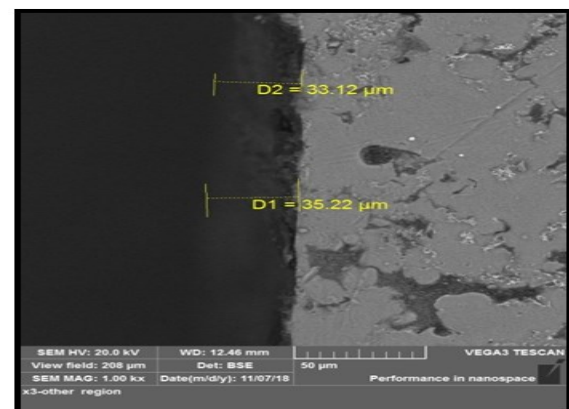
Figure 7: SEM for the Al2024/Al 2 O 3 / Mn composite cladding with SiC powder cross-section
