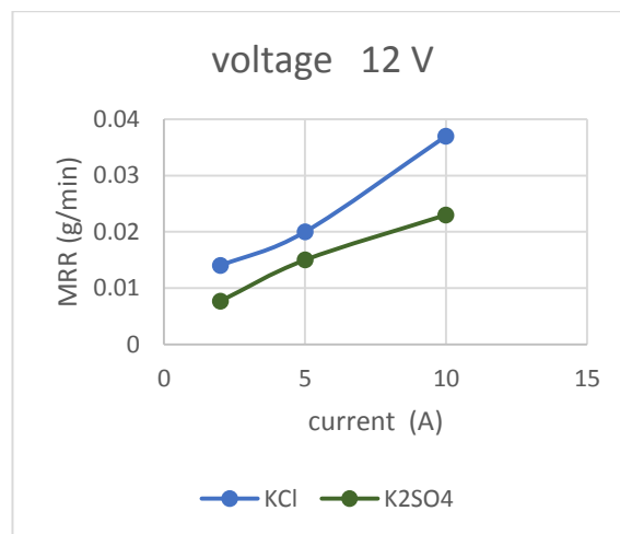
Figure 9: Effect of current on material removal rate at voltage (12V).
