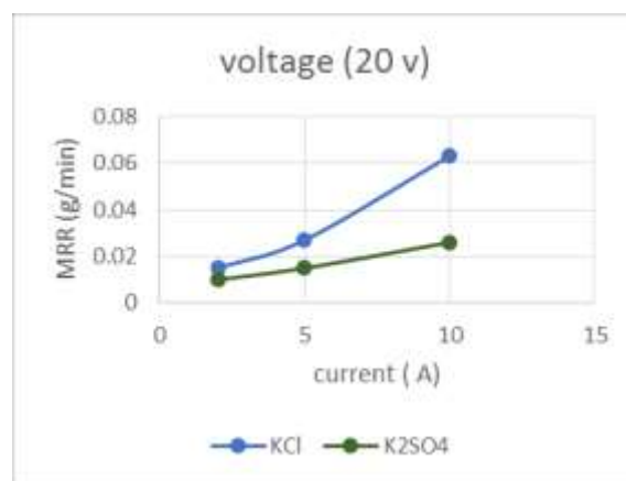
Figure 10: Effect of current on material removal rate at voltage (20) V.
