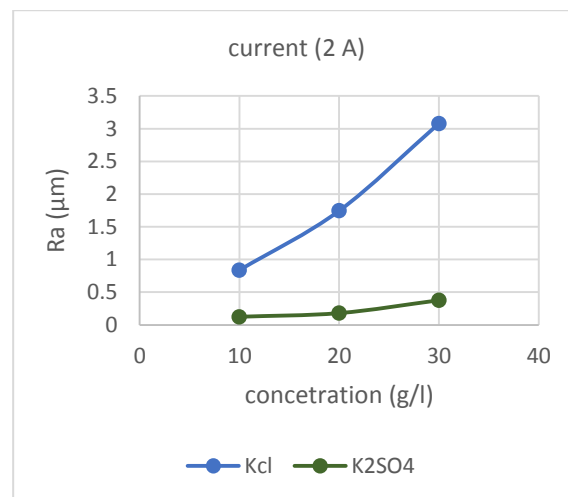
Figure 5: Effect of solution concentration on surface roughness at current (2A)
