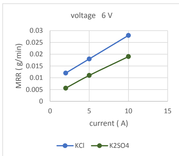
Figure 8: Effect of current on material removal rate at voltage (6V)
