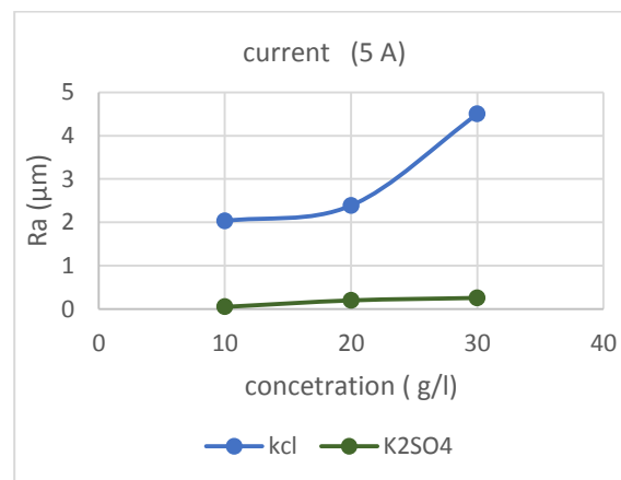
Figure 6: Effect of solution concentration on surface roughness at current (5A)
