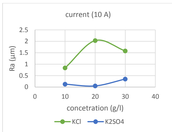
Figure 7: Effect of solution concentration on surface roughness at current (10A)
