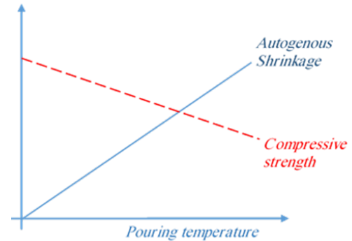
Figure 7: The influence of pouring temperature on autogenously shrinkage and compressive strength
