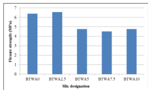
Figure 4: Flexure strength results of black tea waste ash mixes.
