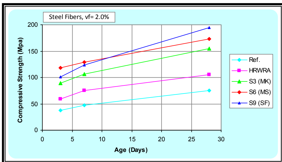
Figure (3): Effect of Pozzolanic Admixture Type on Compressive Strength of RPC Mixes with Steel Fibers
