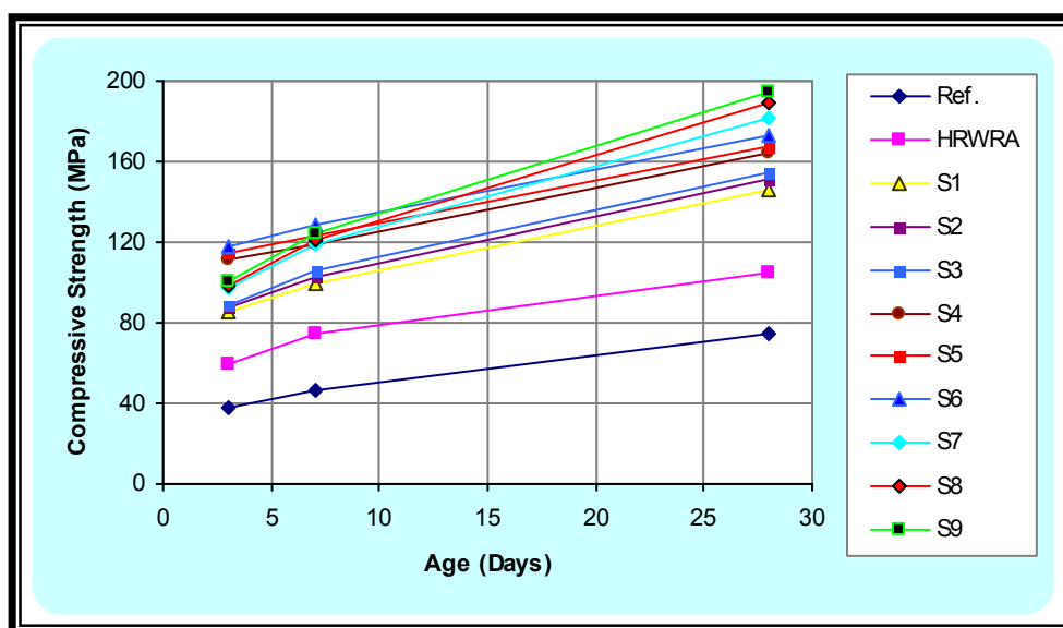
Figure (1): Compressive Strength Development of RPC with Steel Fibers
