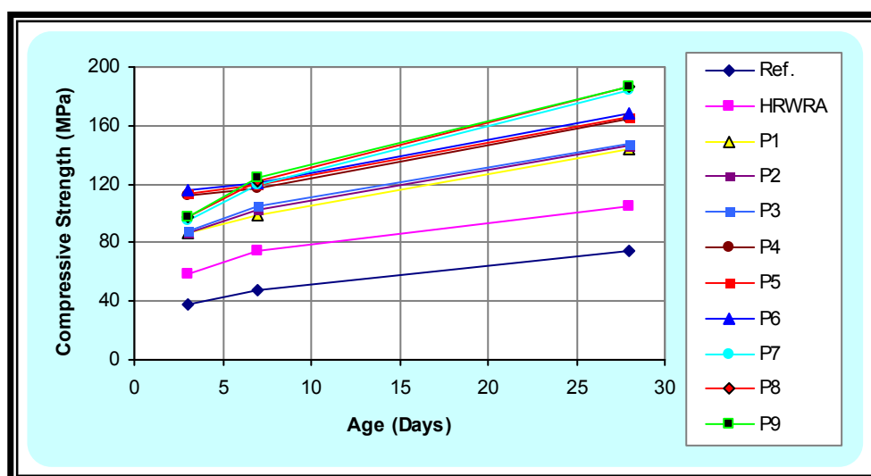
Figure (2): Compressive Strength Development of RPC with Polypropylene Fibers
