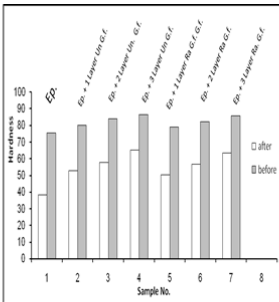
Fig. (1) : The relation between hardness and the type of reinforcing before and after immersion (14 days) in water
