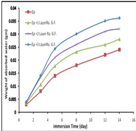
Fig. (5) : the relation between the weight of the absorbed water and the immersion time for samples reinforced by different layers number of random glass fibers.
