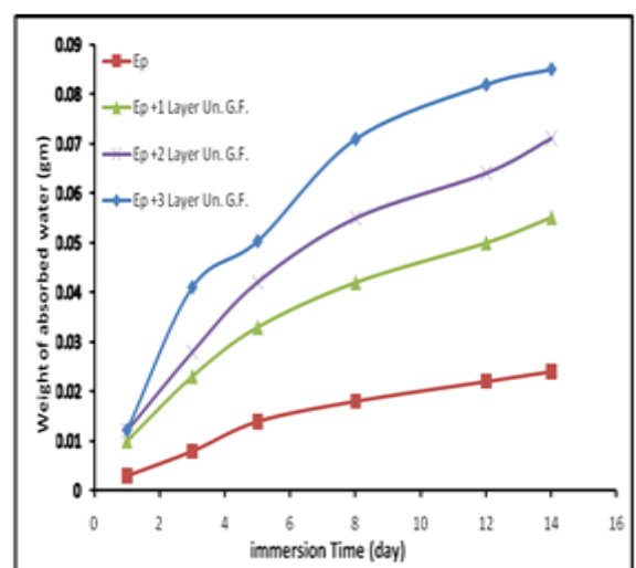
Fig. (4) : the relation between the weight of the absorbed water and the immersion time for samples reinforced by different layers of uniform glass fibers.
