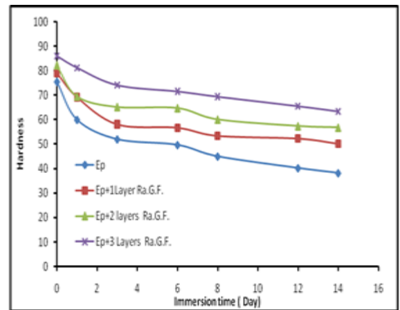
Fig. (3) : The relation between hardness and immersion time in water for samples reinforced with different layers of random glass fiber.
