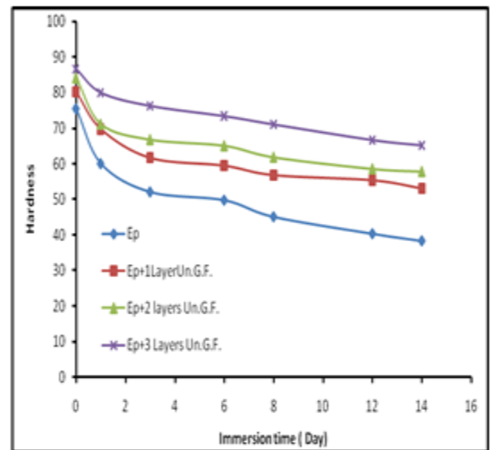
Fig. (2) : The relation between hardness and immersion time in water for samples reinforced with different layers of uniform glass fiber.
