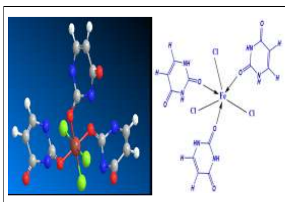
Figure 11: The structure proposed and 3D-geometrical structure of complexes \text{Fe}(\text{Ura})_3\text{Cl}_3
