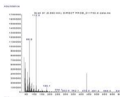
Figure 8: Mass spectrum of [\text{Cr}(\text{Ura})_2(\text{OA})(\text{OH}_2\text{Cl})\cdot\text{H}_2\text{O}] complex
