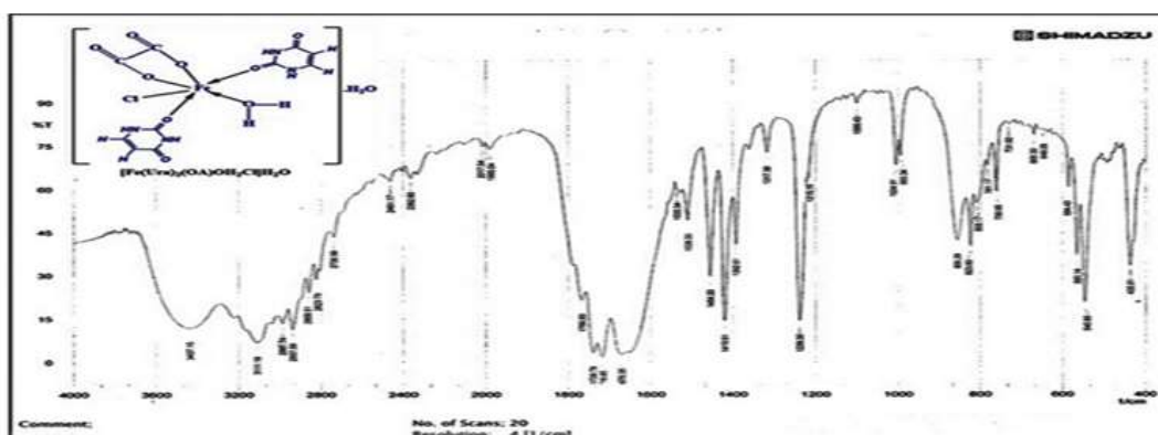
Figure 4: FT-IR spectrum of [\text{Fe}(\text{Ura})_2(\text{OA})\text{OH}_2\text{Cl}]\cdot\text{H}_2\text{O} complex
