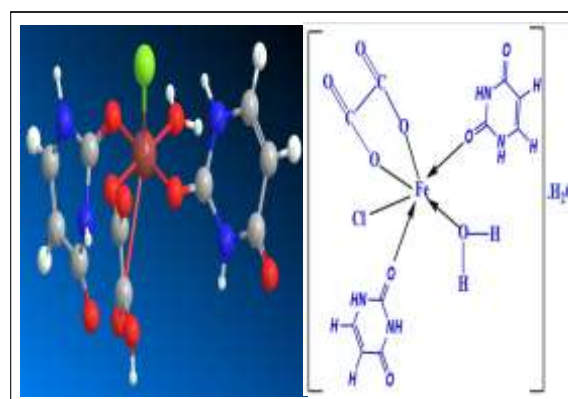
Figure 12: The structure proposed and 3D- the geometrical structure of complexes [\text{Fe}(\text{Ura})_2(\text{OA})(\text{OH}_2)\text{Cl}]\cdot\text{H}_2\text{O}
