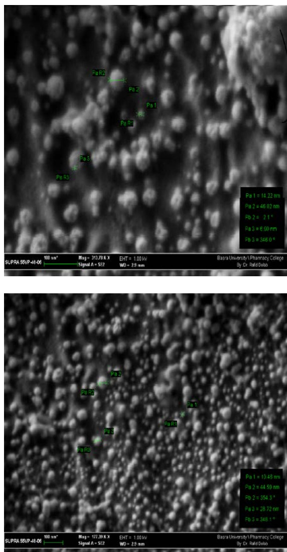
Figure 3: Demonstrations the shape and size of silver nanoparticles prepared by using Indian and Iraqi henna.
