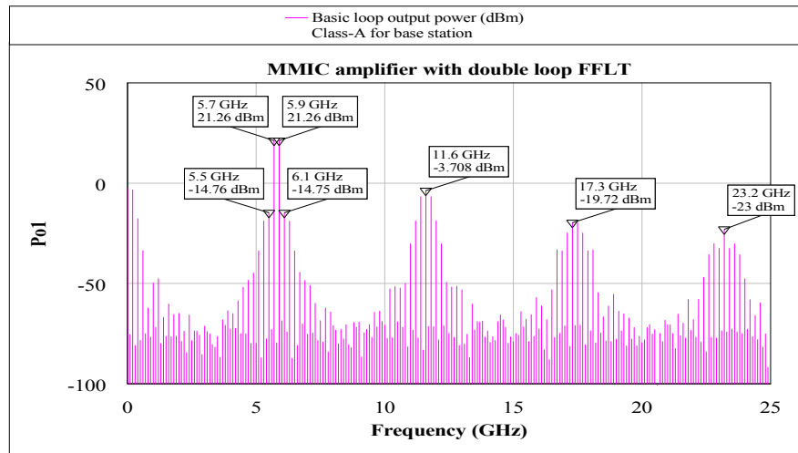
Figure 15. The two-tone test power spectrum of the basic loop in the proposed double loop FFLT with input power level of 5.55 dBm.
