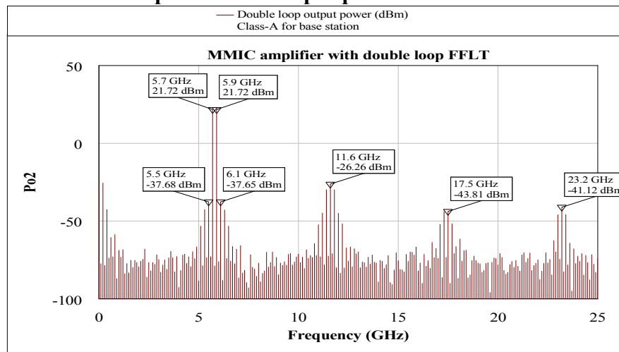
Figure 16. The two-tone test power spectrum of the second loop in the proposed double loop FFLT with input power level of 5.55 dBm.
