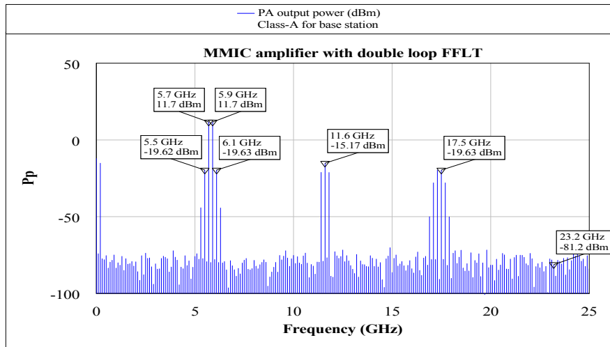
Figure 11. The two-tone test power spectrum of the main amplifier in the proposed double loop FFLT with input power level of -3.98 dBm.
