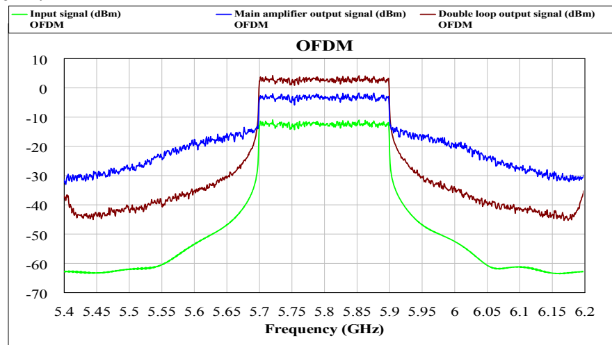
Figure 21. The OFDM response of the proposed double loop FFLT.
