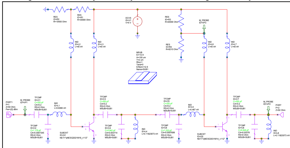
Figure 3. The circuit schematic of class-A PA.
