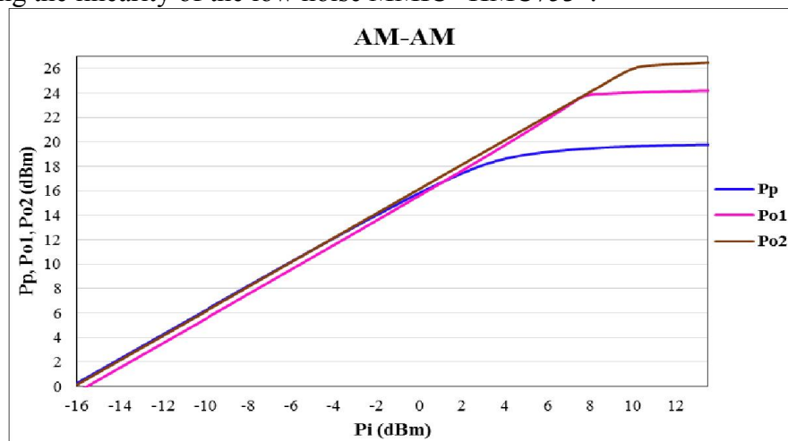
Figure 10. The AM-AM response of the main amplifier, basic loop, and second loop of the proposed double loop FFLT.
