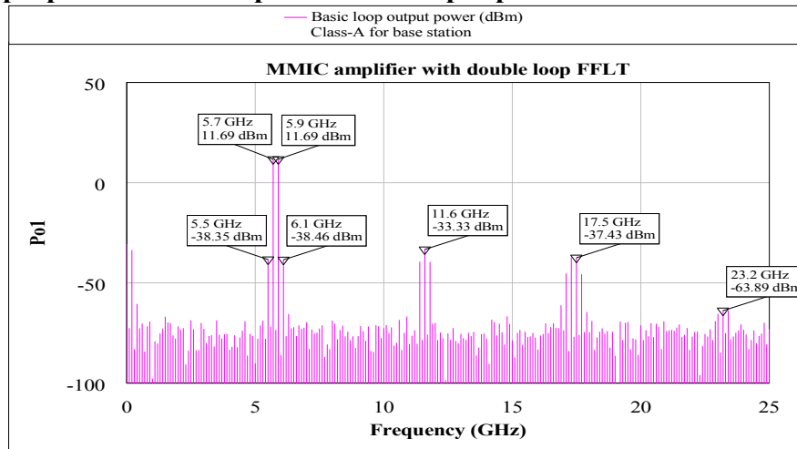
Figure 12. The two-tone test power spectrum of the basic loop in the proposed double loop FFLT with input power level of -3.98 dBm.
