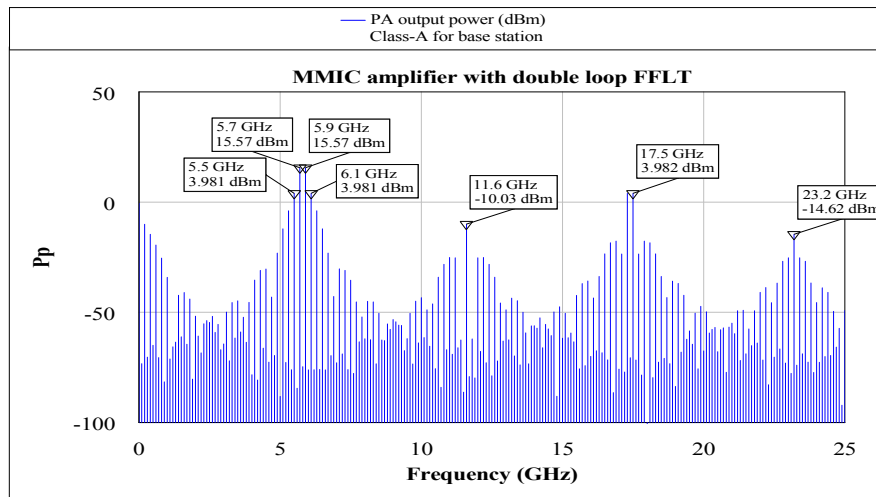
Figure 17. The two-tone test power spectrum of the main amplifier in the proposed double loop FFLT with input power level of 7.4 dBm.
