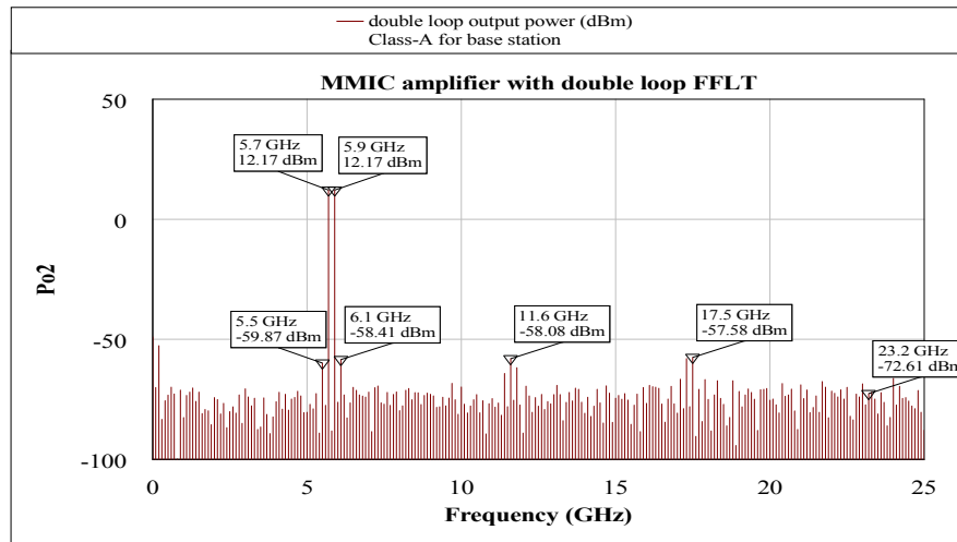
Figure 13. The two-tone test power spectrum of the second loop in the proposed double loop FFLT with input power level of -3.98 dBm.
