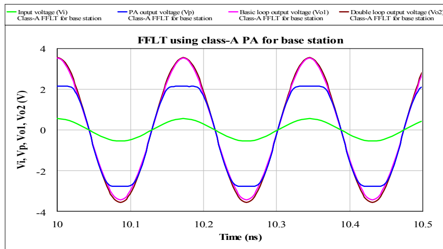
Figure 8. The voltage waveforms of the proposed double loop FFLT with input voltage of 0.55V (peak value).
