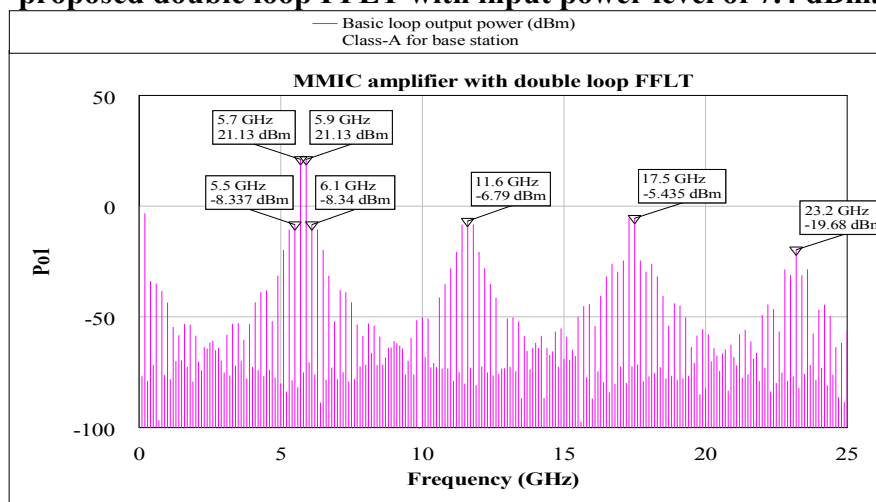
Figure 18. The two-tone test power spectrum of the basic loop in the proposed double loop FFLT with input power level of 7.4 dBm.
