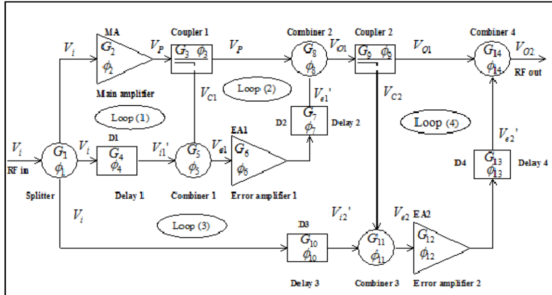
Figure 2. The Double loop FFLT.
