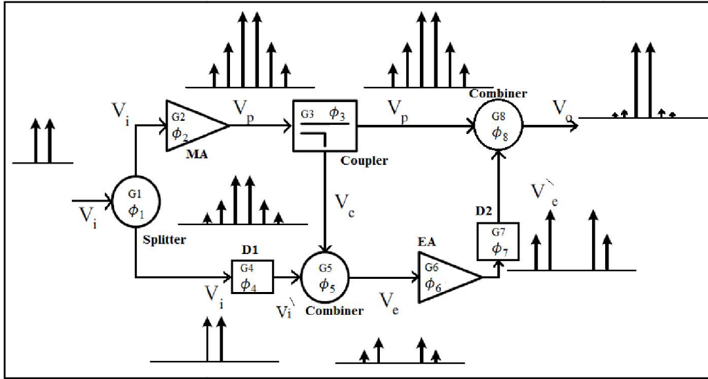
Figure 1. The basic FFLT.
