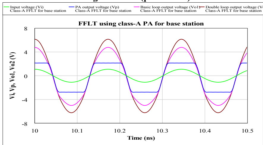
Figure 9. The voltage waveforms of the proposed double loop FFLT with input voltage of 1.1V (peak value).
