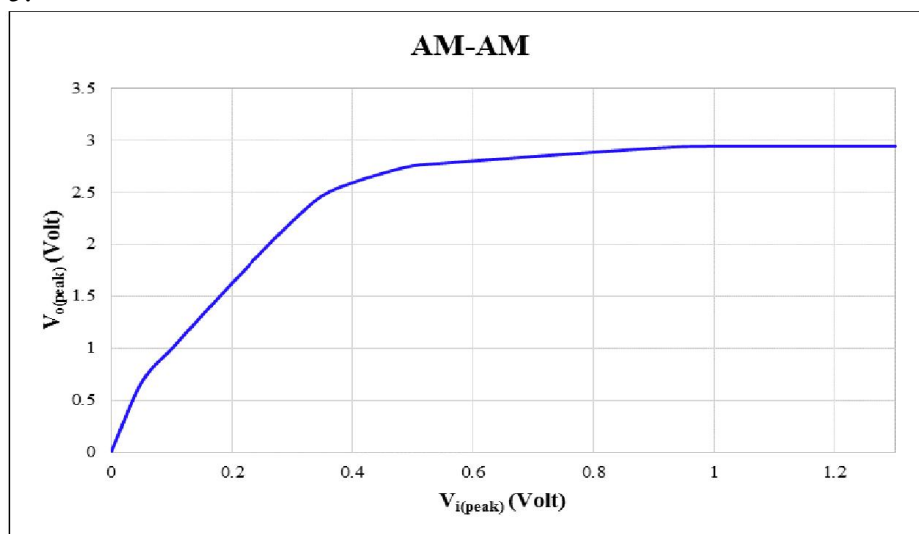
Figure 5. The AM-AM characteristics of the MMIC “HMC753” amplifier at an operating frequency of 5.8 GHz.
