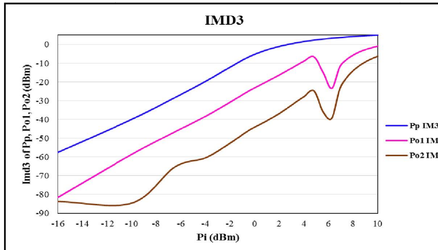
Figure 20. The IMD3 of the main amplifier, the basic loop, and double loop FFLT using class-A power amplifiers.
