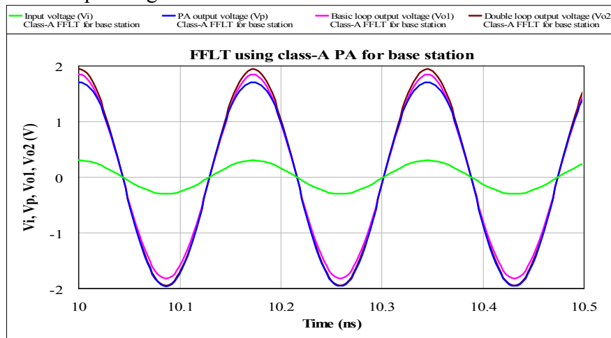
Figure 7. The voltage waveforms of the proposed double loop FFLT with input voltage of 0.3V (peak value).
