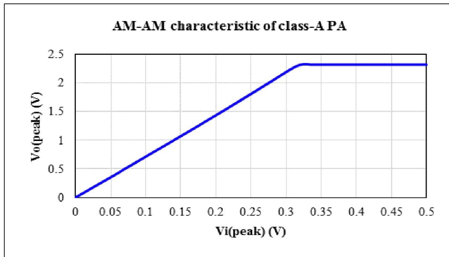
Figure 6. AM-AM characteristics of the proposed class-Aerror amplifier.
