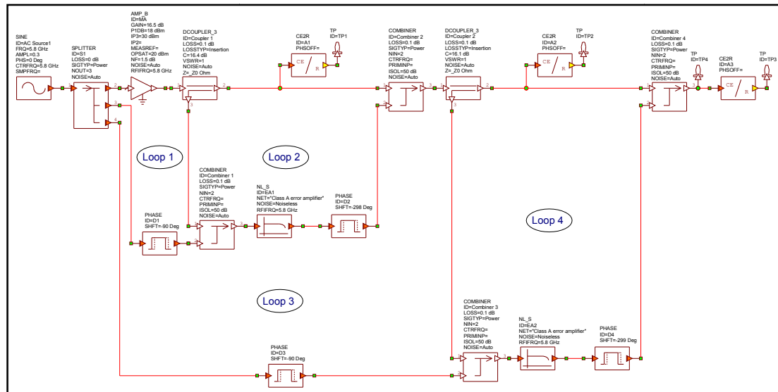
Figure 4. The circuit diagram of the proposed double loop FFLT system for linearizing a MMIC low noise amplifier using a 2-stage class-A power amplifier as error amplifier.
