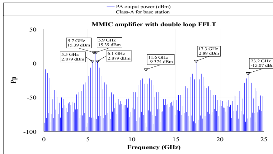
Figure 14. The two-tone test power spectrum of the main amplifier in the proposed double loop FFLT with input power level of 5.55 dBm.
