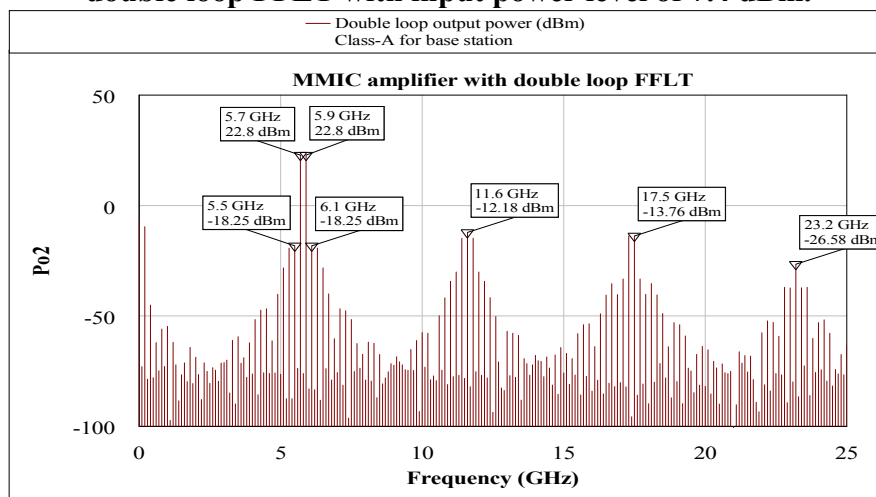
Figure 19. The two-tone test power spectrum of the second loop in the proposed double loop FFLT using class-A power amplifiers with input power level of 7.4 dBm.
