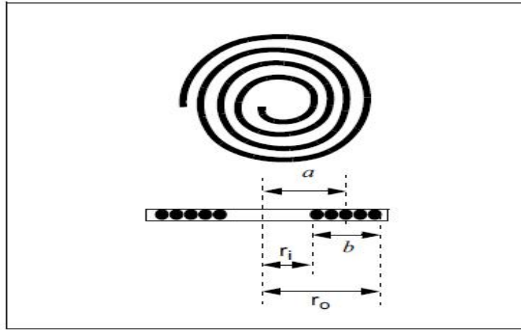
Figure 5.The spiral coil.
