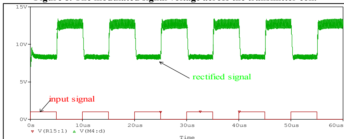
Figure 9. Rectifier output voltage.
