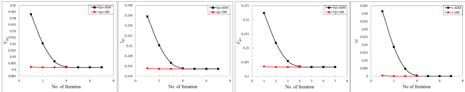
Fig. 4 – Existence results of numerical techniques for non-Linear equation.
