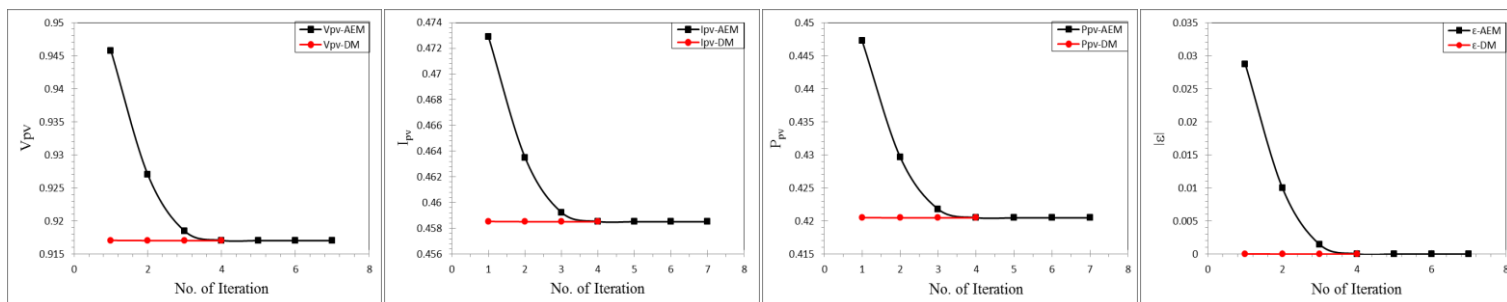
Fig. 2 – Existence results of numerical techniques for non-Linear equation.
