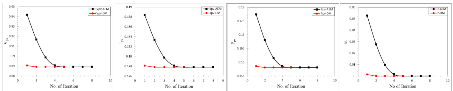
Fig. 5 – Existence results of numerical techniques for non-Linear equation.
