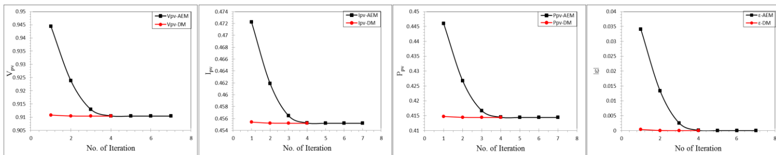
Fig. 3 – Existence results of numerical techniques for non-Linear equation.
