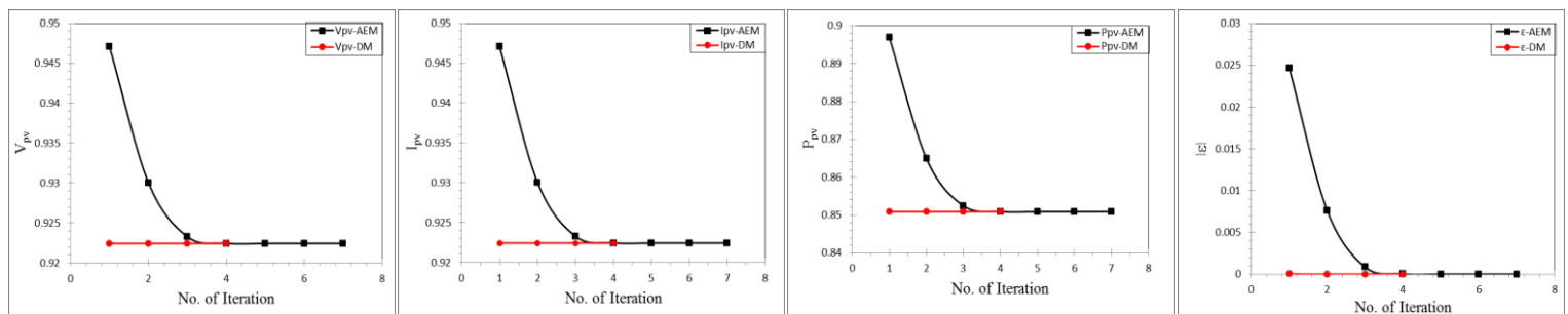
Fig. 1 - Existence results of numerical techniques for non-Linear equation.
