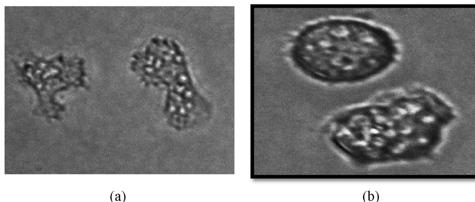
Fig. 2. Image of morphological structure of cells under light microscopy observation for (a) untreated cells has trophozoite active form, irregular shape with existence of acanthapodia and vacuoles, and (b) treated cells showing a dormant cyst form, round shape and decrease in size, structure of acanthapodia shorten or lost, cyst formed under unfavourable environmental conditions caused the encystment of the cells. Magnification was 400x.
