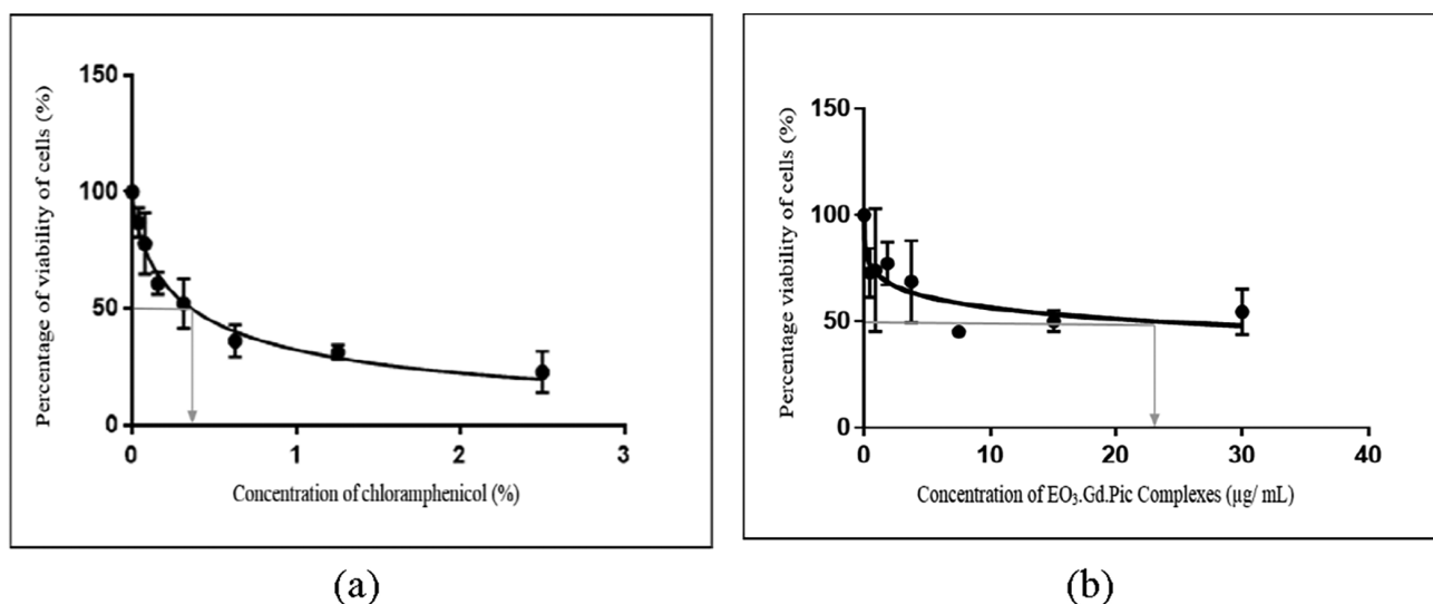
Fig. 1. Comparison of percentage viability of cells assessed by using MTT assay after 24 hours exposed to chloramphenicol with the IC 50 value of 0.39 (%) (a), and (b) percentage viability of cells assessed by using MTT assay after 24 hours exposed to the Gd complex with the IC 50 value of 23.44 μg/mL.
