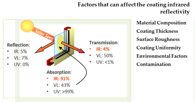
Fig. 4. interaction of solar spectrum components (IR, Visible, and UV) with thin window films.
