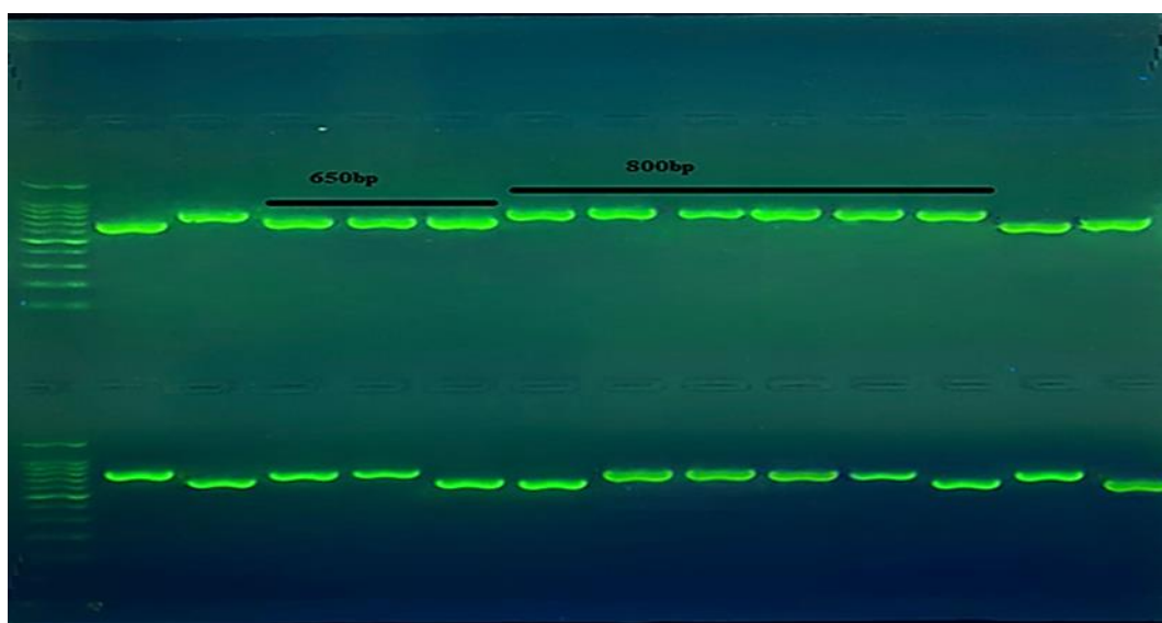
Figure 4.2 Uni21/Lmj4 PCR result with a band size of 800 bp. Electrophoresis on 2% agarose at 5 volt/cm2 produced the final product.
