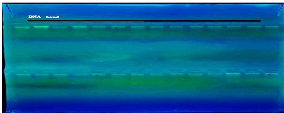
Figure 4.1 Gel electrophoresis of genomic DNA extraction from samples in 1% agarose gel for 30 min
