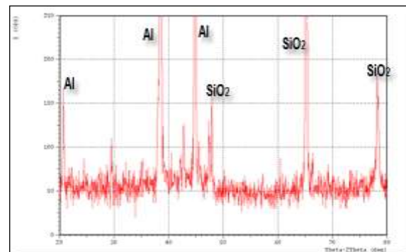
Figure 6: X-Ray diffraction analysis of hybrid composite Al alloy+ 2 wt%B 4 C+ 15 wt% fly ash
