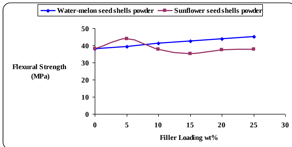
Fig.(1): The effect of filler loading of water-melon and sunflower seed shells powder on flexural strength of unsaturated polyester.
