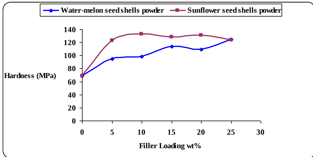
Fig.(6): The effect of filler loading of water-melon and sunflower seed shells powder on hardness of unsaturated polyester.
