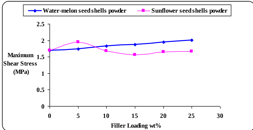
Fig.(3): The effect of filler loading of water-melon and sunflower seed shells powder on maximum shear stress of unsaturated polyester.
