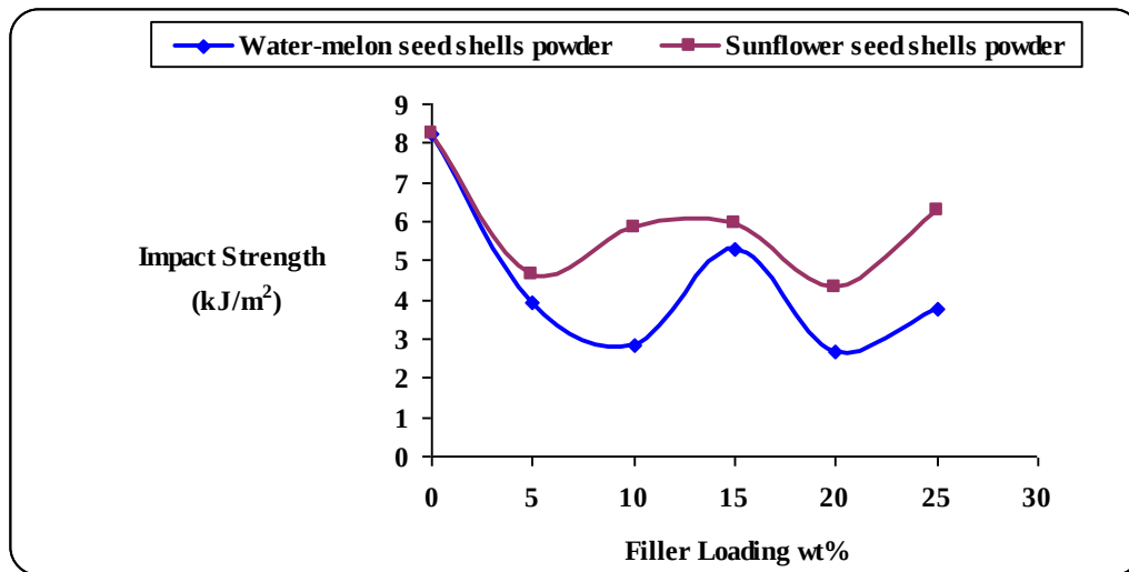
Fig.(4): Variation of the impact strength of polyester with filler loading of shells powder.
