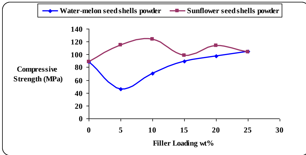
Fig.(5): The effect of filler loading of water-melon and sunflower seed shells powder on compressive strength of unsaturated polyester.
