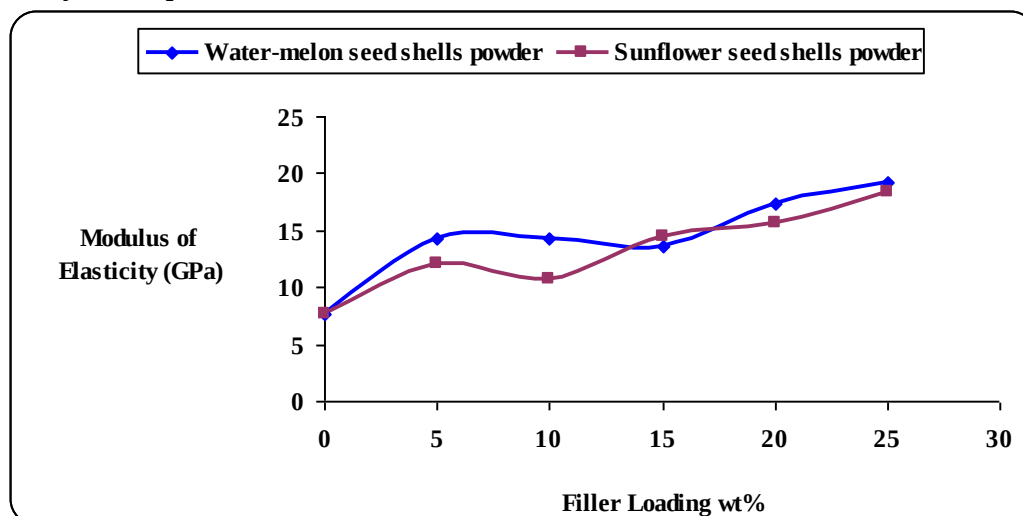
Fig.(2): The effect of filler loading of water-melon and sunflower seed shells powder on modulus of elasticity of unsaturated polyester.
