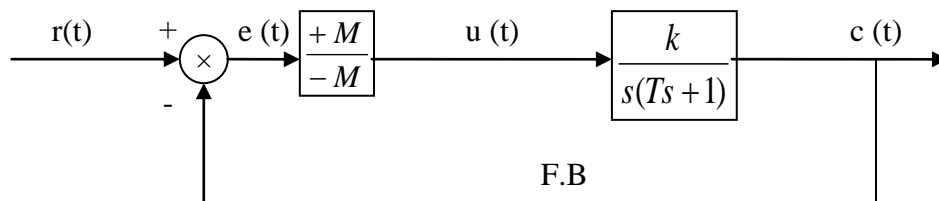
Fig (1-b) A simplified on-off servo system
