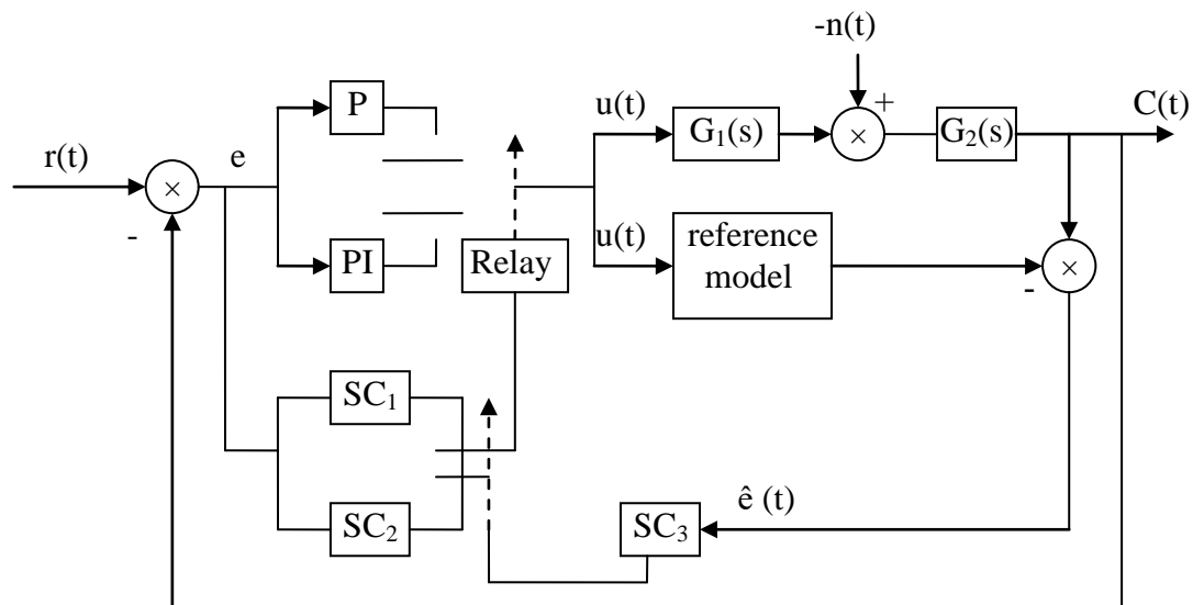
Fig (9) adaptive VSS using (P&amp;PI) controller
