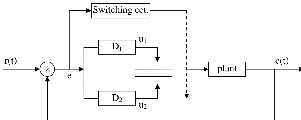
Fig (6) block diagram (p) and (PI) controller for switching circuit with VSS. [Ogata, K, 2005].
