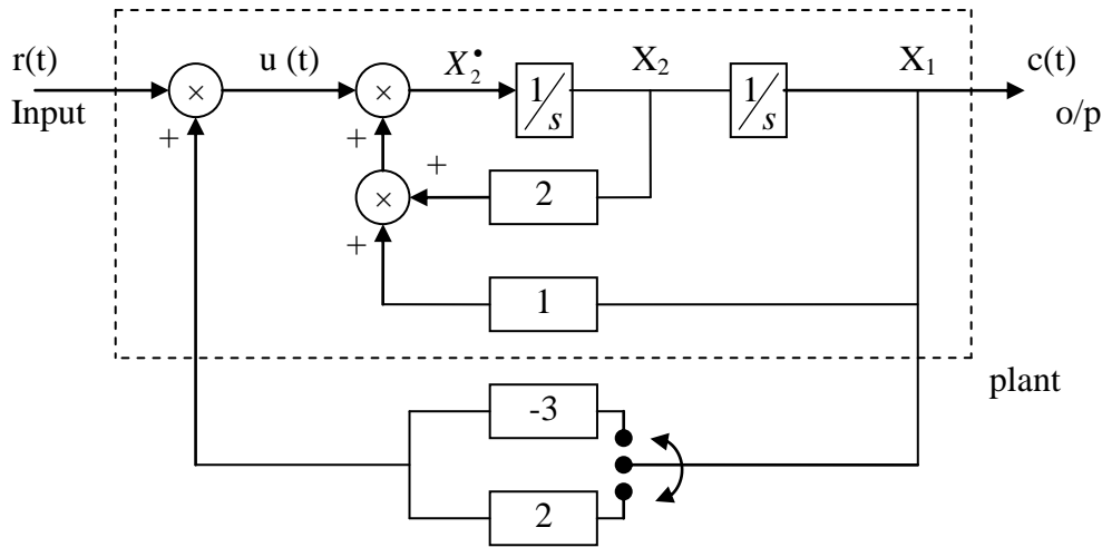
Fig (4) simplified block diagram by linear structure for (VSC) in the plant system.
