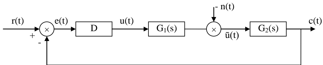
Fig (5) control system under disturbance.
