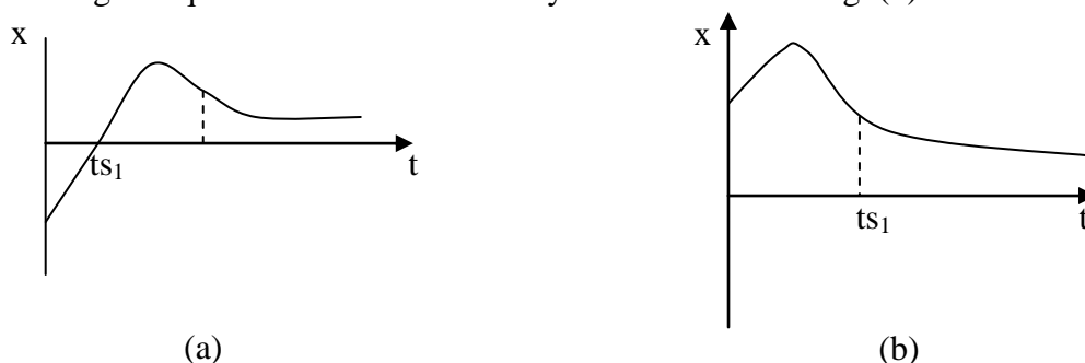
Fig (3) shows two moment of switching conditions with VSC plant
