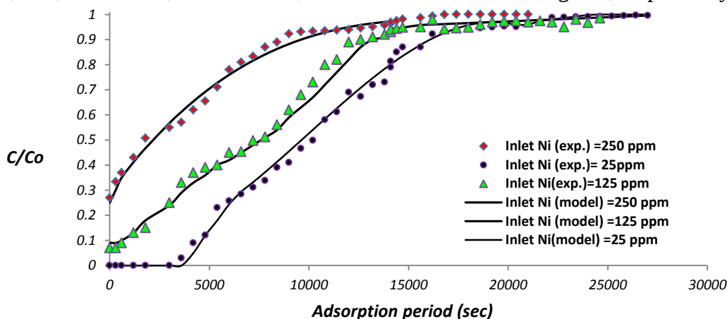
Figure 7: The Experimental and model results for Nickel removal at various initial concentrations
