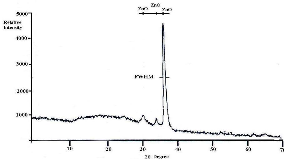
Figure (3) The XRD pattern of the prepared samples at O_2 pressure of 300 mbar and substrate temperature 423K.
