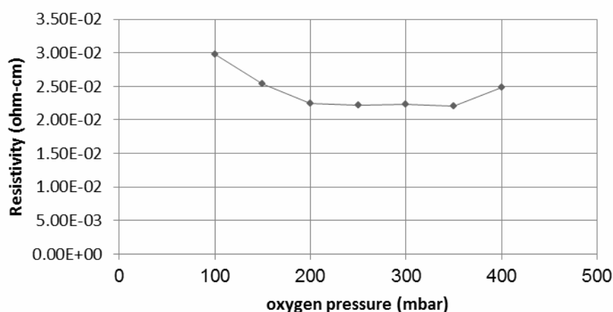
Figure (1) Resistivity vs. \text{O}_2 pressure for Zn samples
