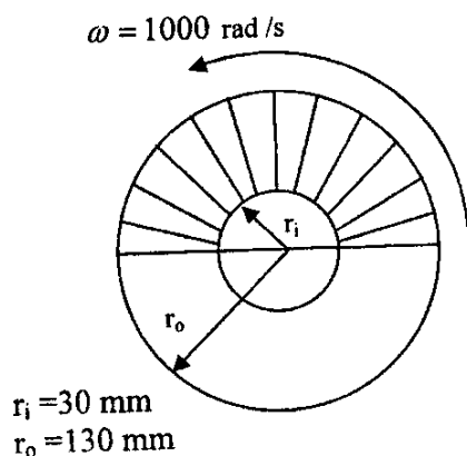
A – Radial fiber reinforced disc.
