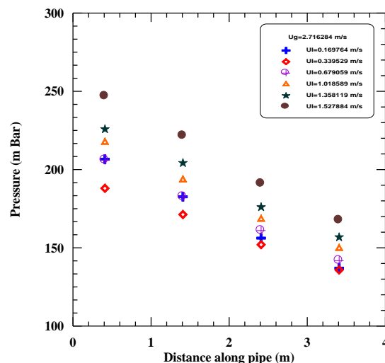
Figure (17) relation between pressure and distance along pipe for various superficial velocity with ( Q_v=20 l/min)
