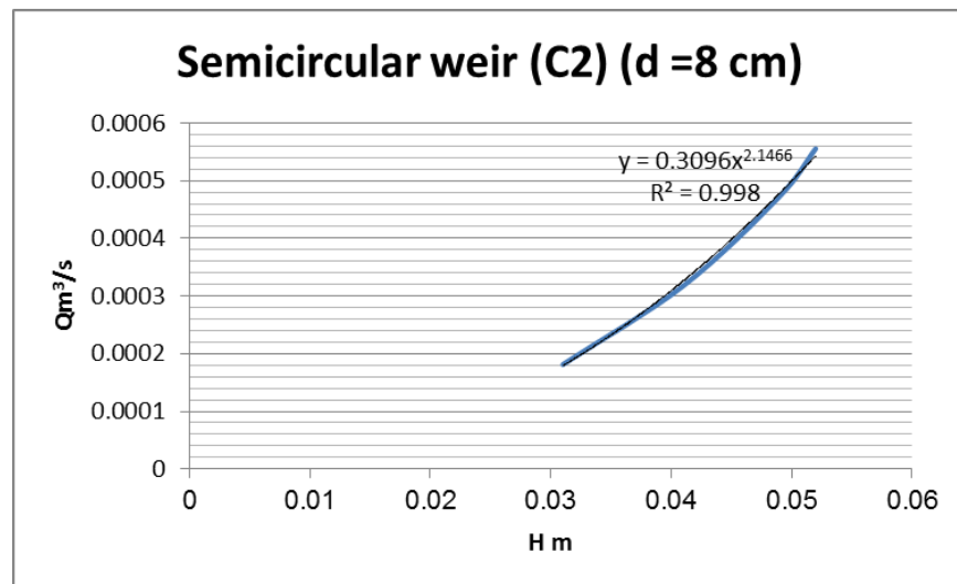
Fig (6) Rating semicircular weir (d=8cm).
