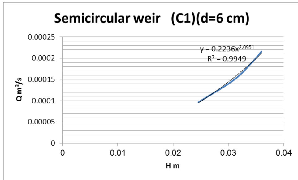
Fig (5) Rating of semicircular weir (d=6 cm).
