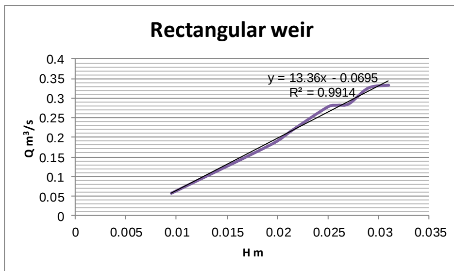
Fig (3) Rating rectangle weir.
