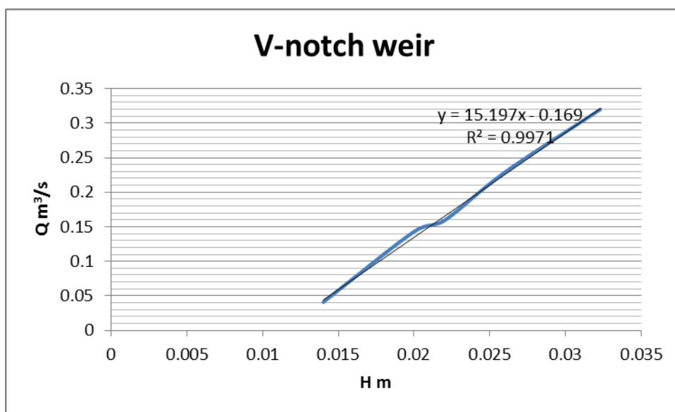
Fig (4) Rating v- notch weir.
