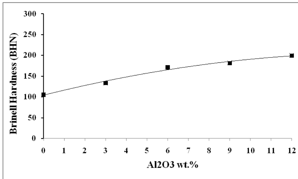
Fig. 5: Illustrate the relation between concentration of \alpha -alumina particles and Brinell hardness (BHN).
