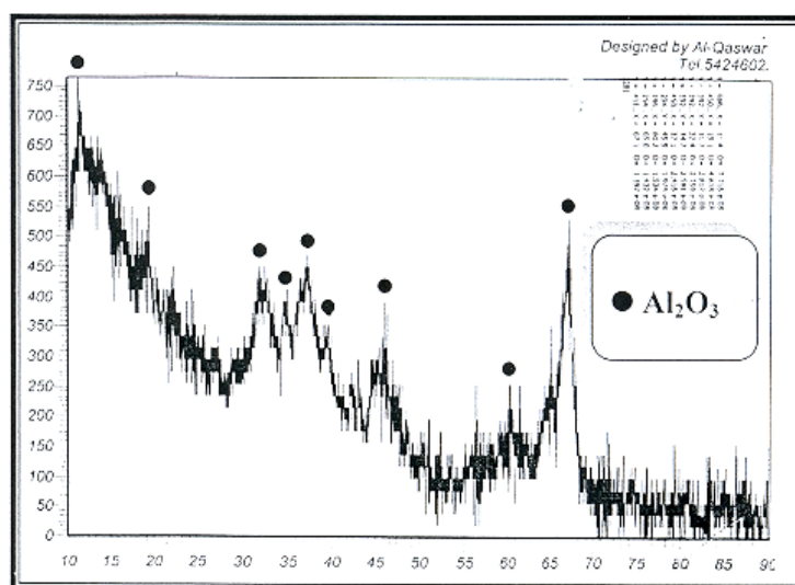
Fig. 1: Diffractograms from the surface of \alpha -( \text{Al}_2\text{O}_3 ) particles.
