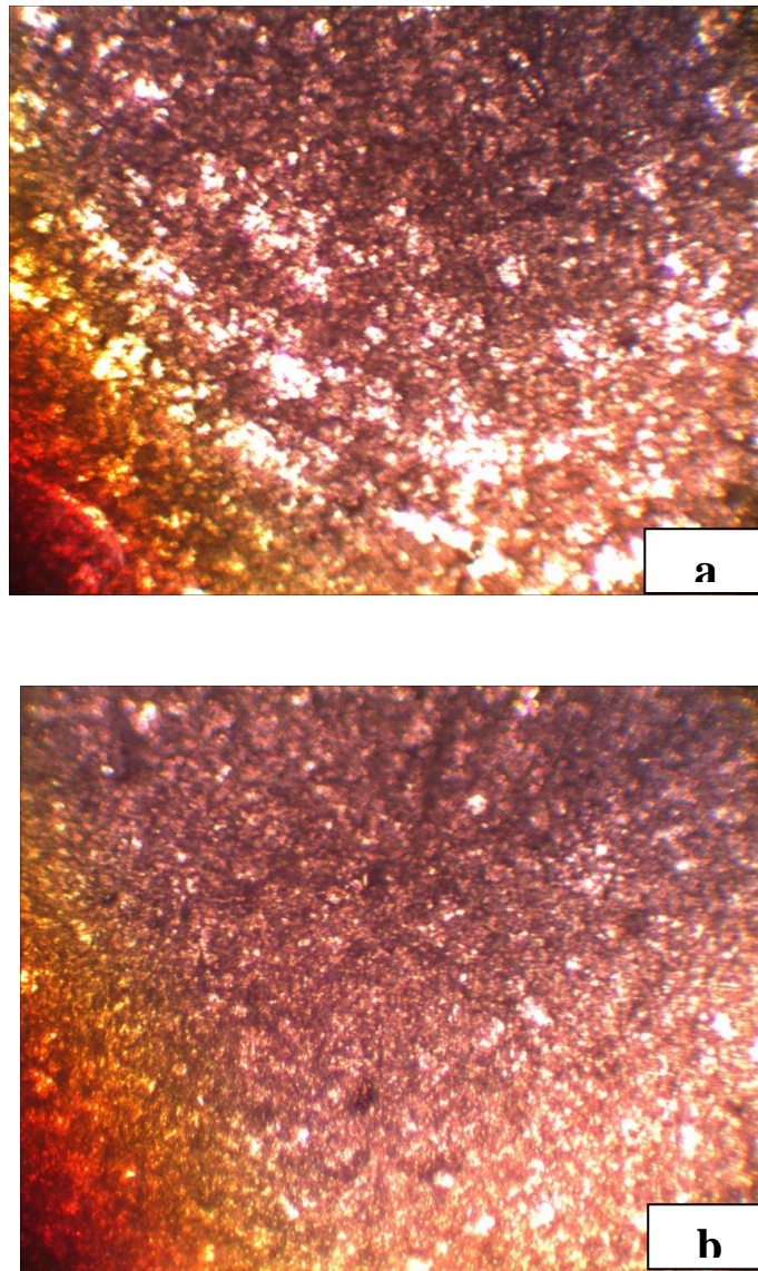
Fig. 4: light optical micrograph for as polished aluminum reinforced by 12wt.% \alpha -Al 2 O 3 particles (a) before sintering process, (b) after sintering process Alumina particles appear darker than the aluminum matrix.
