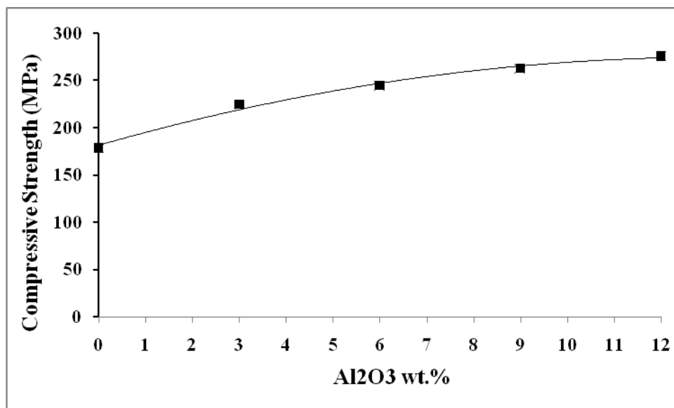
Fig. 6: Illustrate the relation between concentration of \alpha -alumina particles and Compression strength (MPa).
