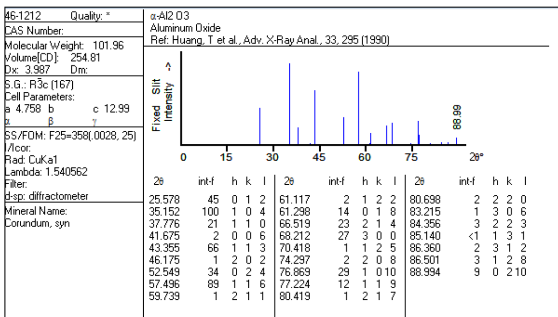
Fig. 2: Standard Diffractograms of \alpha - \text{Al}_2\text{O}_3
