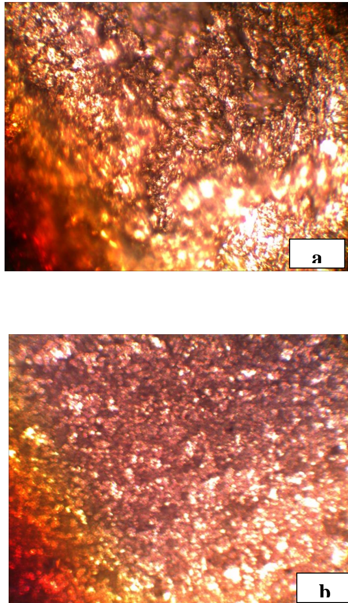
Fig. 3: light optical micrograph for as polished aluminum reinforced by 6 wt.% \alpha -Al 2 O 3 particles (a) before sintering process, (b) after sintering process Alumina particles appear darker than the aluminum matrix.
