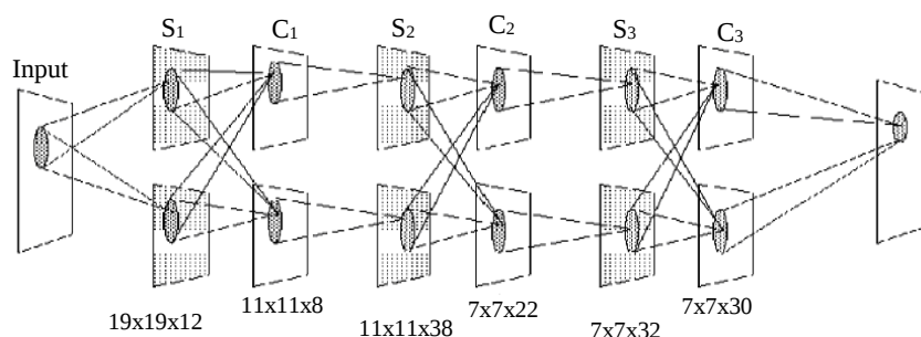
Figure 2. Layout of Neocognitron
