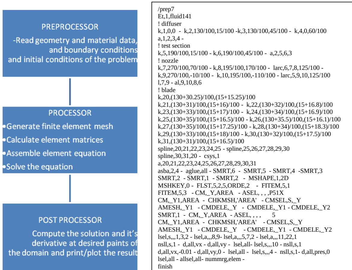
Fig. (15): Flow chart and APDL for numerical Simulation
