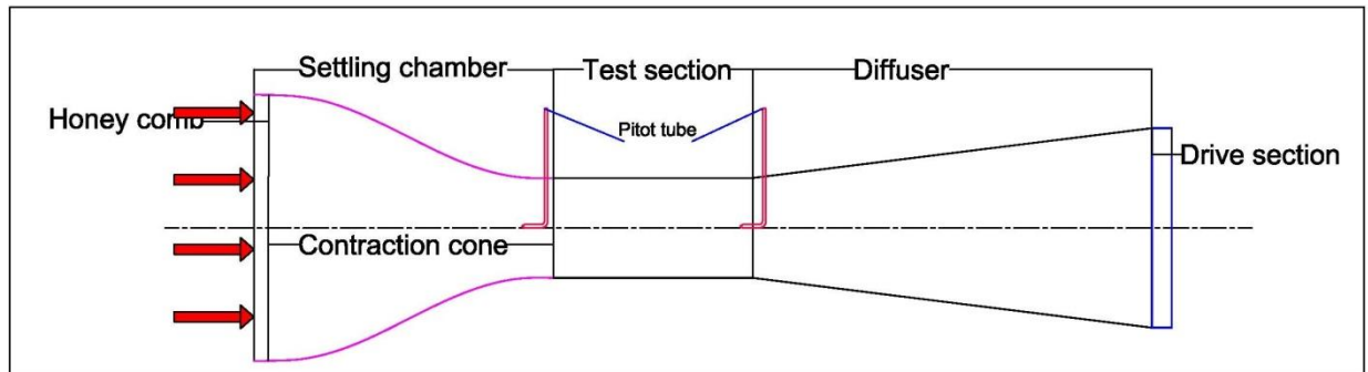
Fig (13) Schematic of wind tunnel shown the pitot tube position
