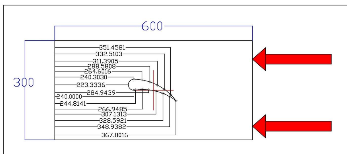
Fig(11) The mounted of the specimen
