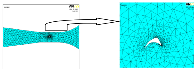
Fig.(17) Mesh of wind tunnel
