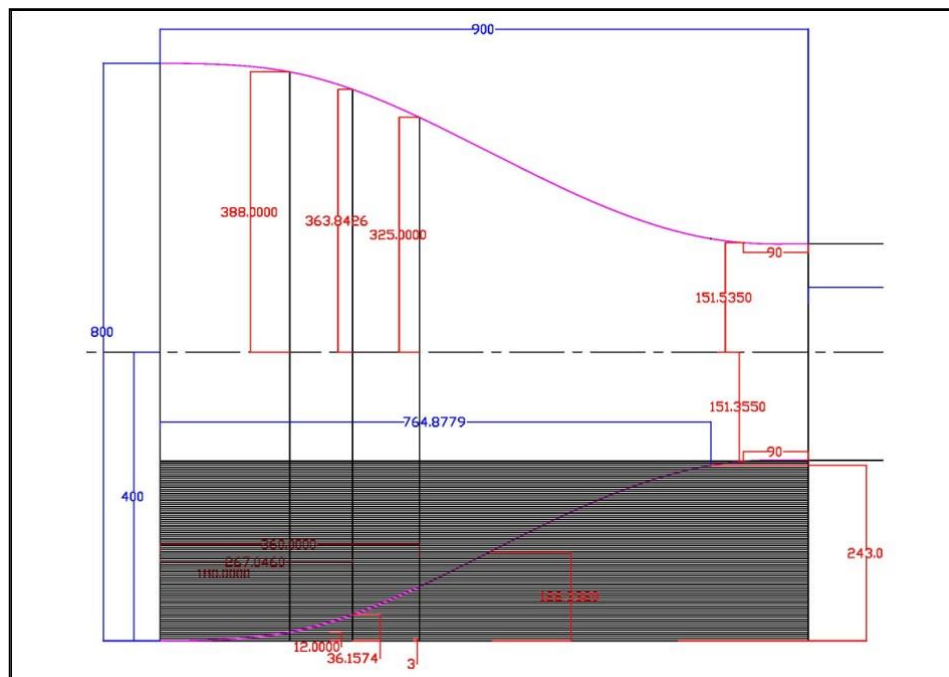
Fig. (5) settling chamber
