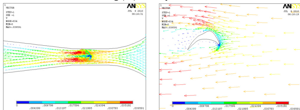
Fig.(21) velocity vector
