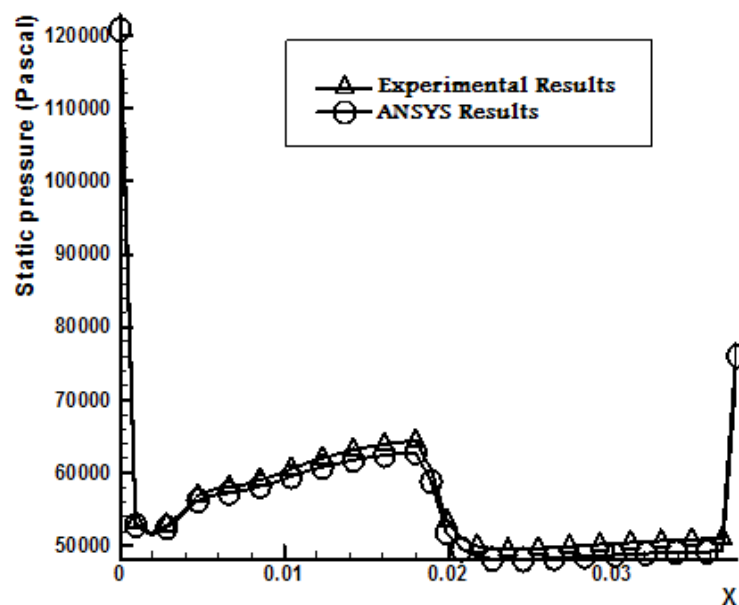
Fig.(18) Static pressure distribution on the upper surface
