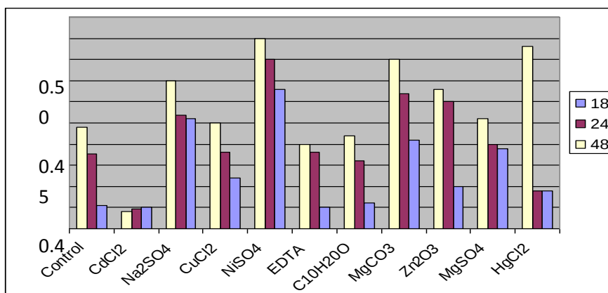
Figure 1: show the absorbance of pigments in broth media of P. aeruginosa
