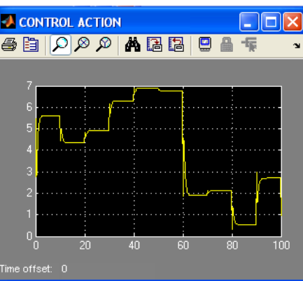
Figure (17): control Action
