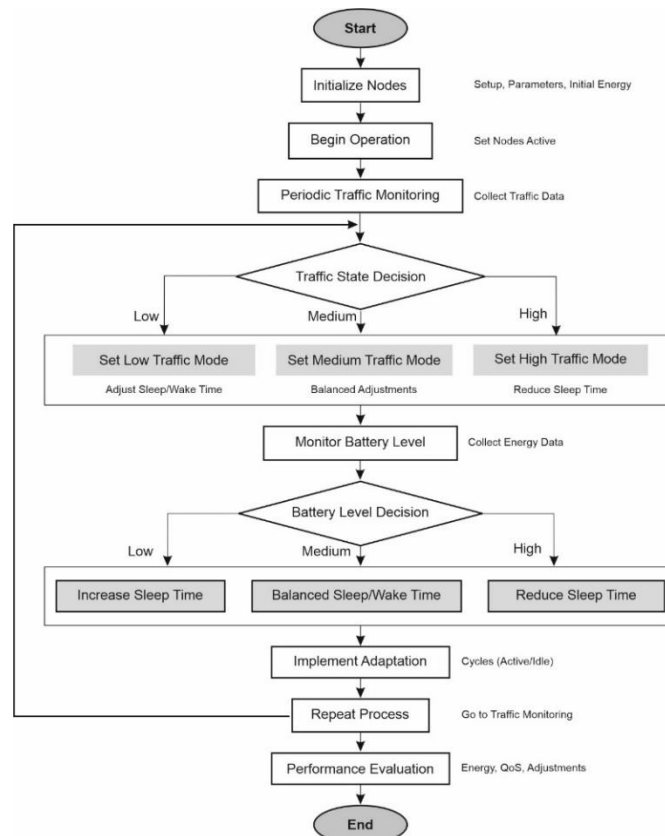
FIGURE 1. - Visually illustrates the main steps of the algorithm.
