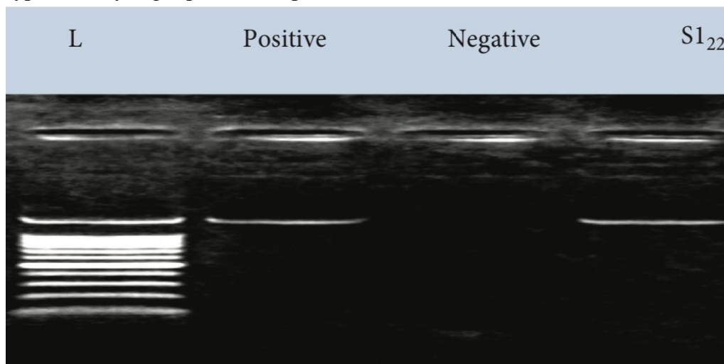
Figure 1: Gel electrophoresis of the PCR product of the isolated probiotic strain, where lane 1, molecular weight ladder; lane 2, a positive control; lane 3, a negative control; and lane 4 (S1), the specific DNA product of about 1485 base pairs (bp) amplified from the isolate.
