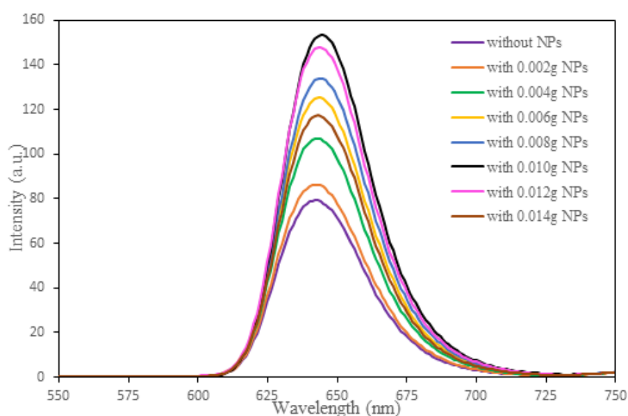
Fig. (5) The fluorescence intensity with amount of \text{SiO}_2 nanoparticles
