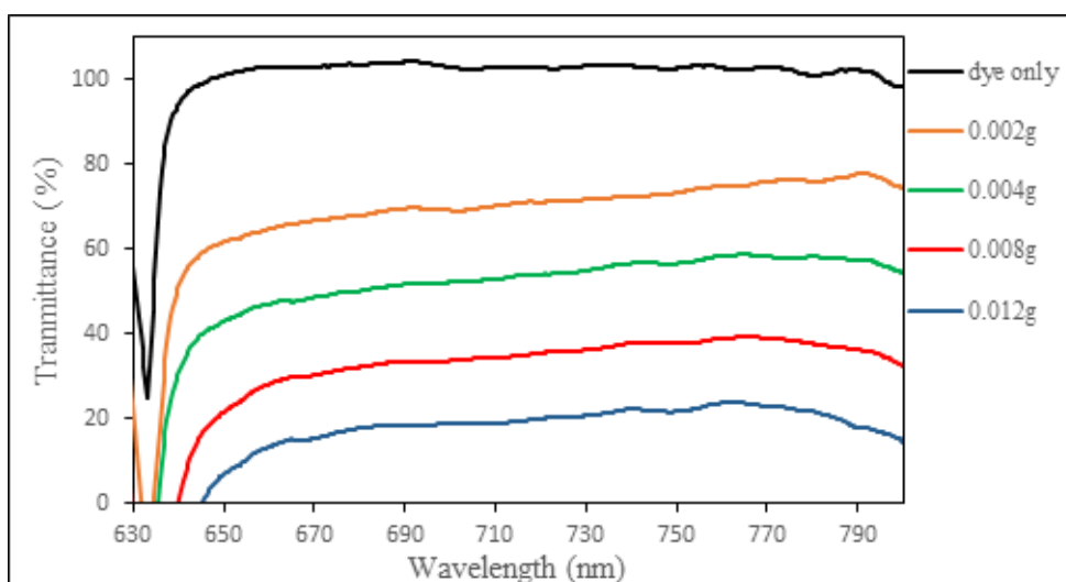
Fig. (3) The transmission spectra at different concentrations of Rhodamine B dye dissolved in water with amount of \text{SiO}_2 nanoparticles.
