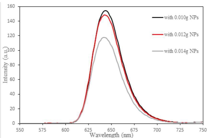
Fig. (6) Behavior of \text{SiO}_2 nanoparticles quenching with Rhodamine B dye
