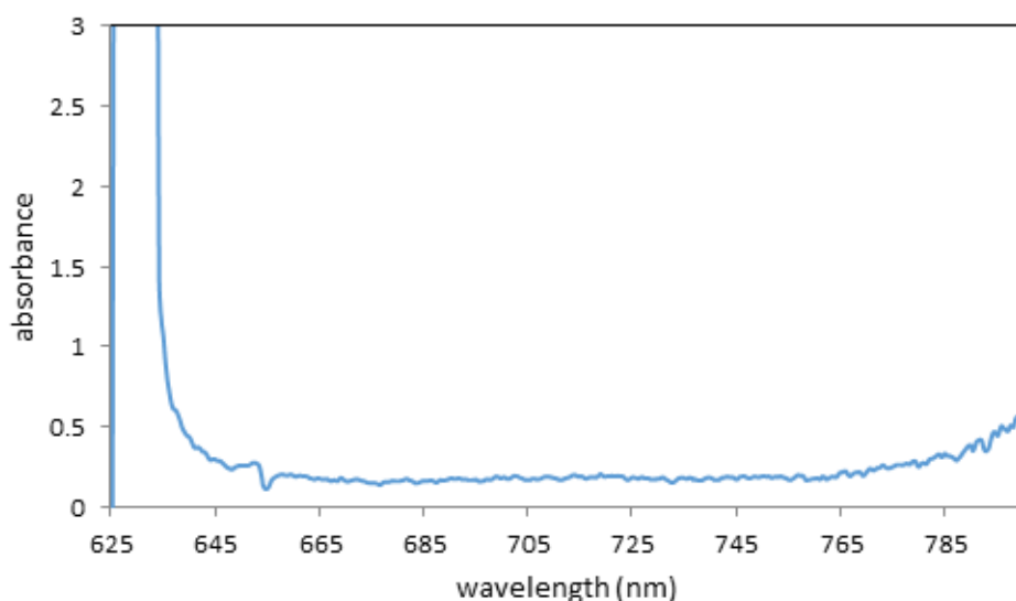
Fig. (1) The absorption spectrum of the Rhodamine B dye with, 5 \times 10^{-3} \text{M} concentration dissolved in water.
