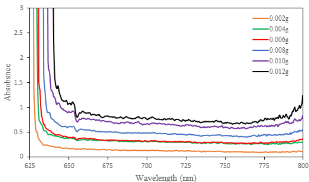
Fig. (2) The absorption spectra of 5 \times 10^{-3} \text{M} Rhodamine B dye solution with different amounts of \text{SiO}_2 nanoparticles
