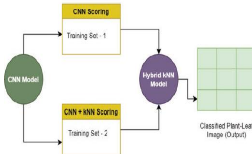
Figure 6: (Hybrid CNN-KNN)Classification
