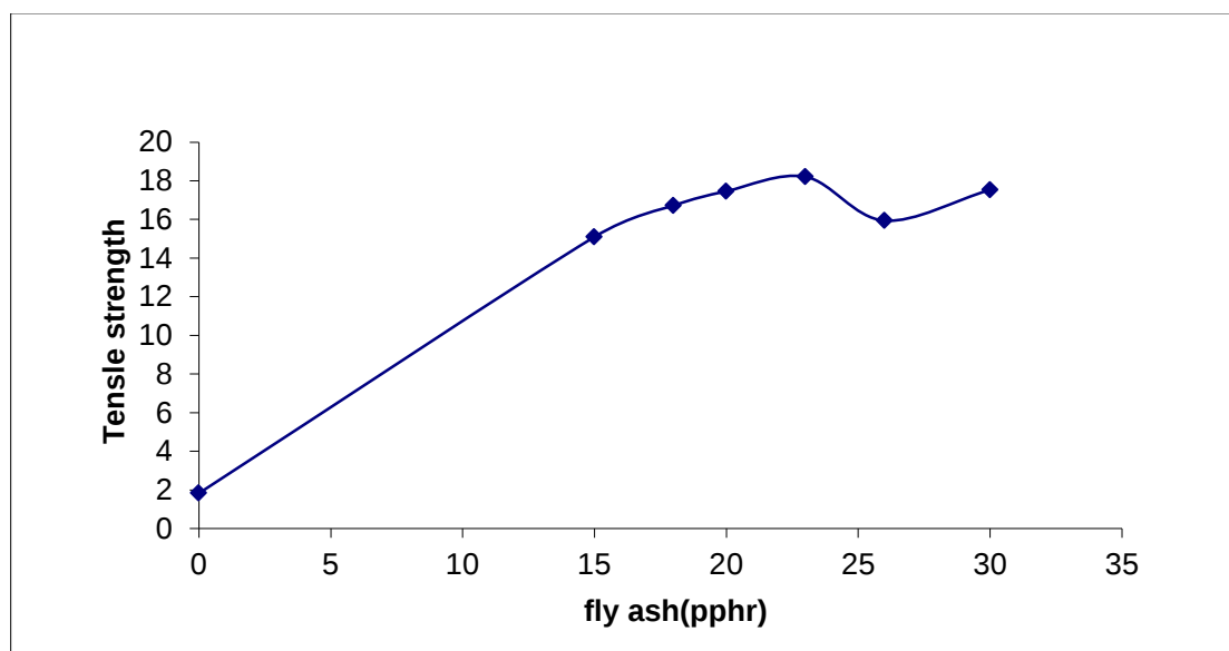
Figure(2) Effect of adding waste of cement on tensile strength
