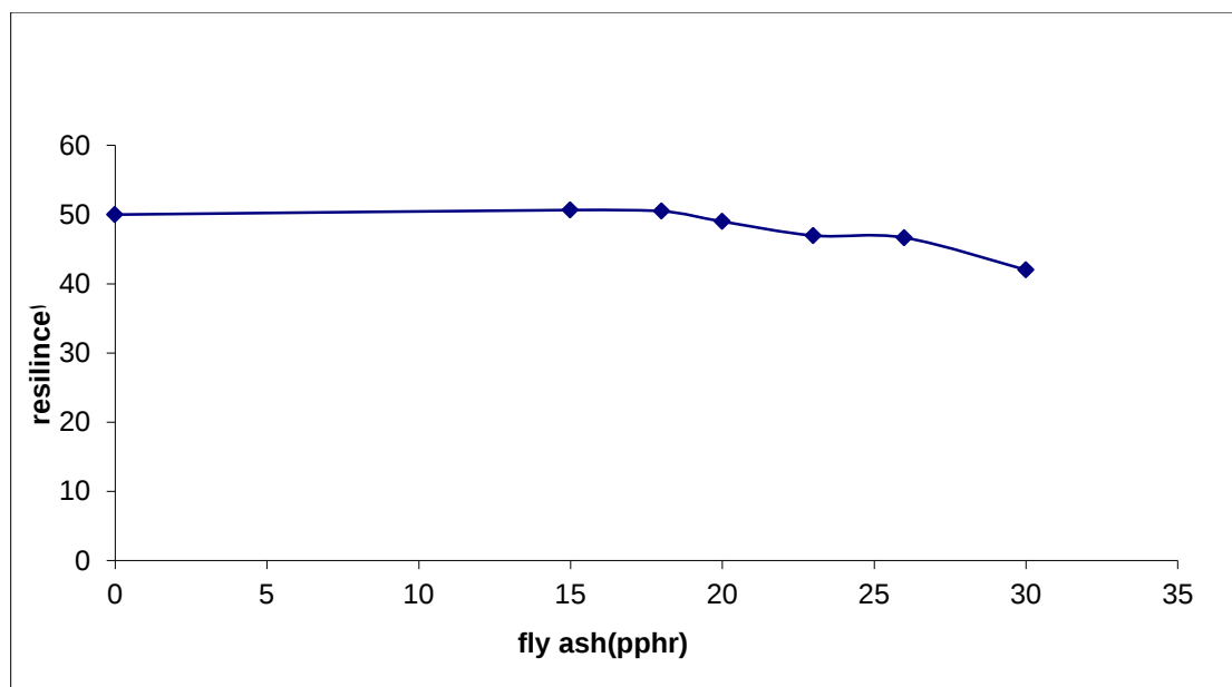
Figure(7) effect of adding waste of cement on resilience
