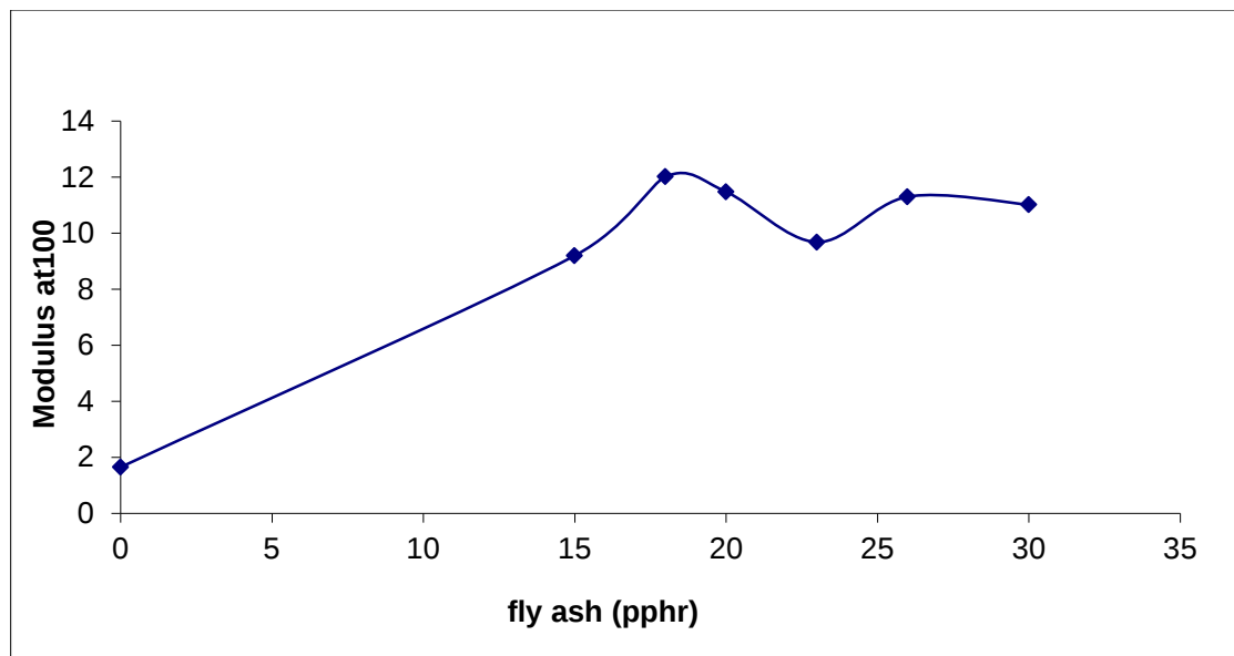
Figure(3) effect of adding waste of cement on modulus
