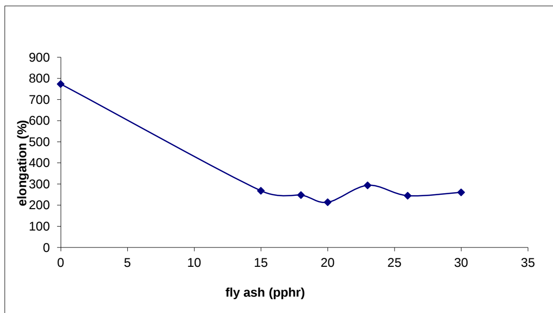
Figure(4) effect of adding waste of cement on elongation
