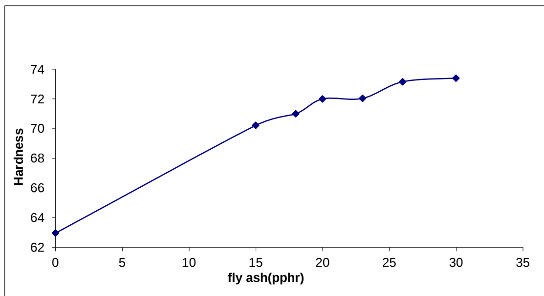
Figure(6) effect of adding waste of cement on hardness
