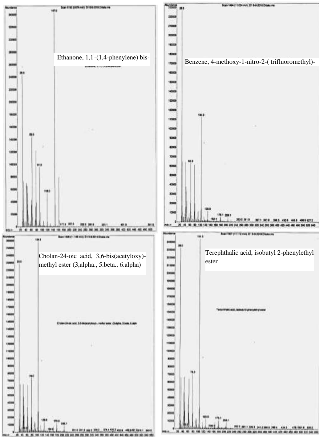
Fig.4a: The compounds of crude chloroform extract produced by the dried methanol pulverized Conocarpus leaves detected by GC-MS analysis.
