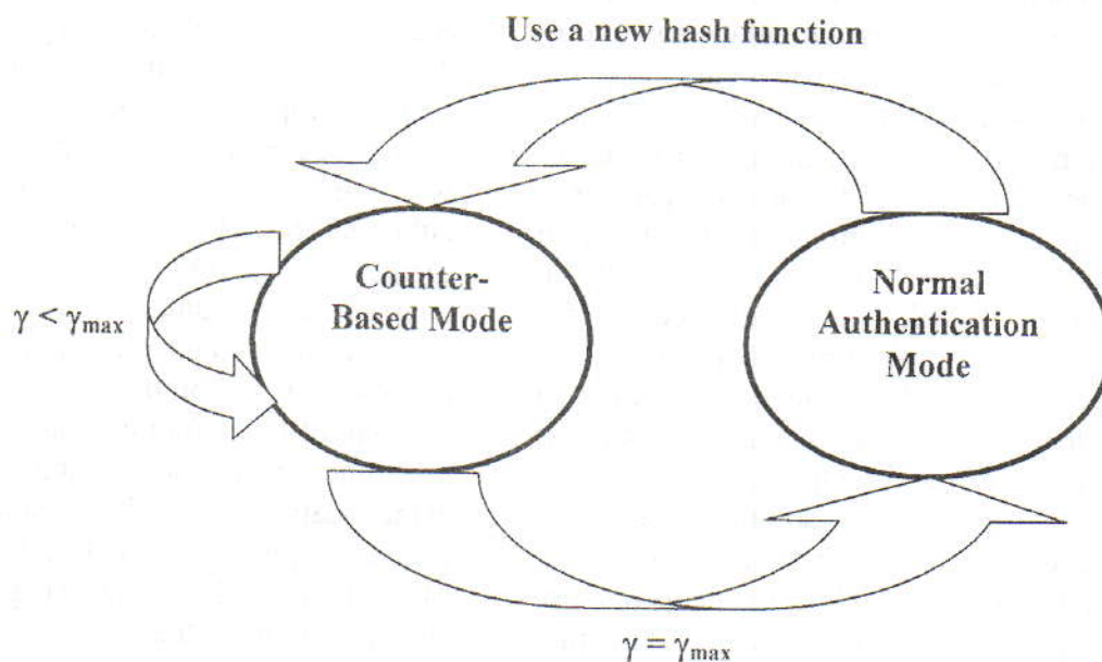
Figure 2: A state diagram for the proposed hybrid authentication strategy
