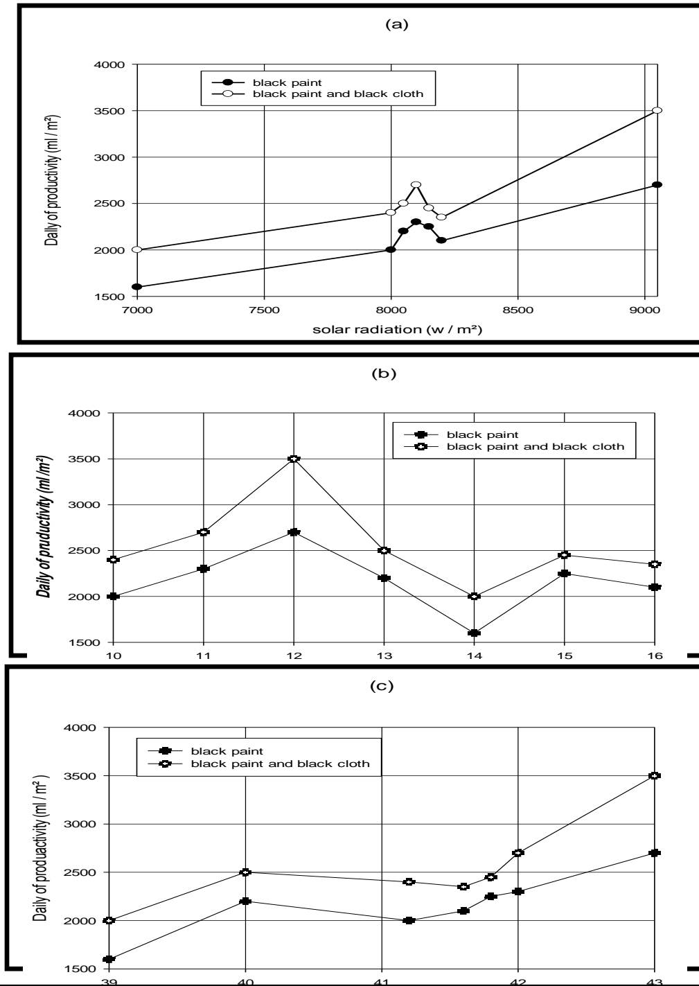
Fig.2: (a) Show relationship Between daily production of the two double slope solar still and solar radiation . (b) The productivity with the days of the test . (c) the productivity with Temperature of the test days .
