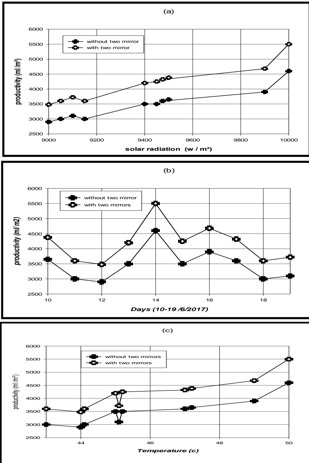
Fig 6: (a) daily production of the two double slope solar still and solar During (10- 19 /6/2017). (b) The productivity with the days of the test . (c) the productivity with Temperature of the test days .
